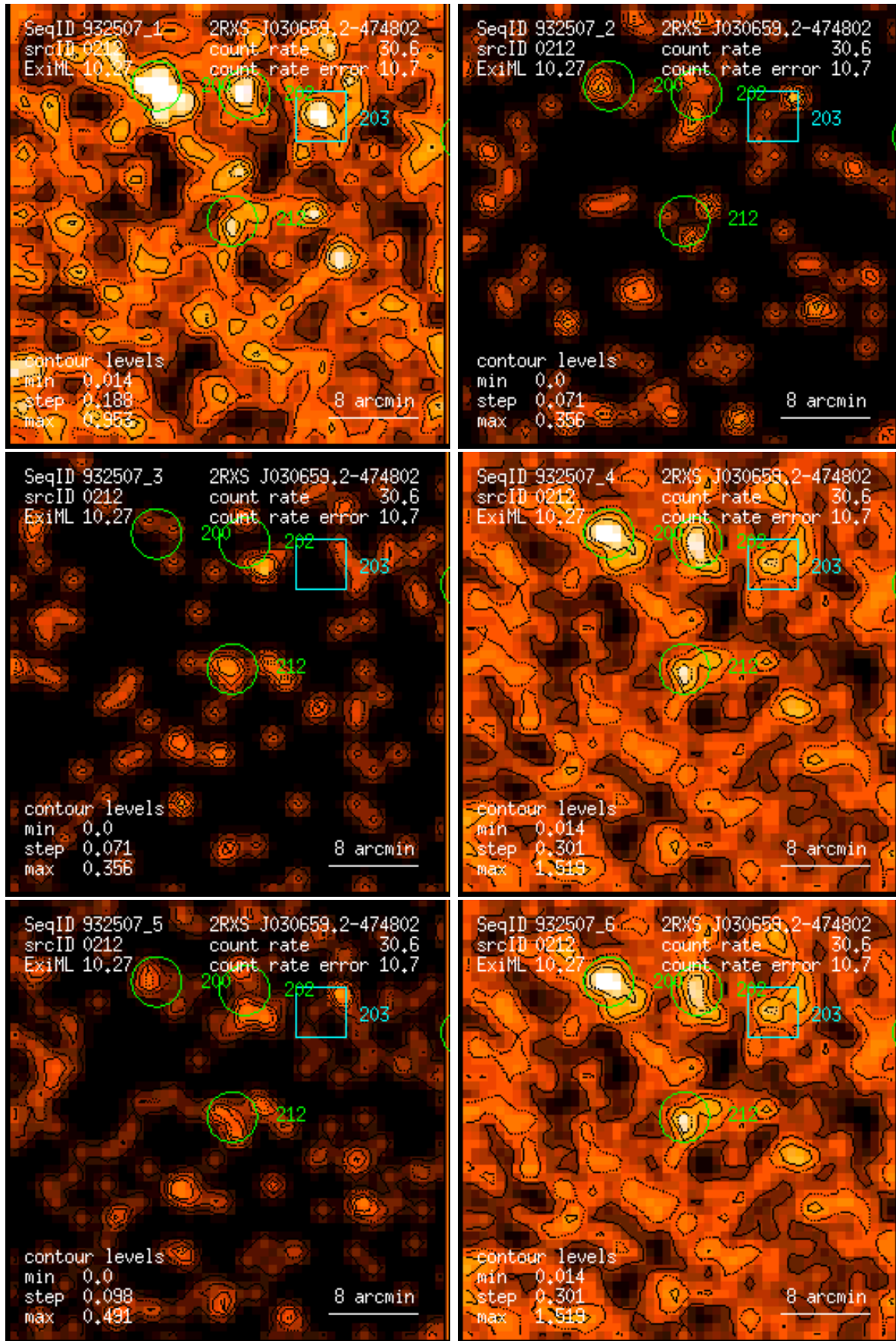
Figure 212: RASS 932507: detection 0212: band rate images, Gaussian filter: (1) PSPC channels 11 – 41, (2) 52 – 90, (3) 91 – 201, (4) 11 – 235, (5) 52 – 201, (6) 11 – 201. Broad band rates in counts/ks. Band rate contour levels in counts/ks/arcmin 2 .
