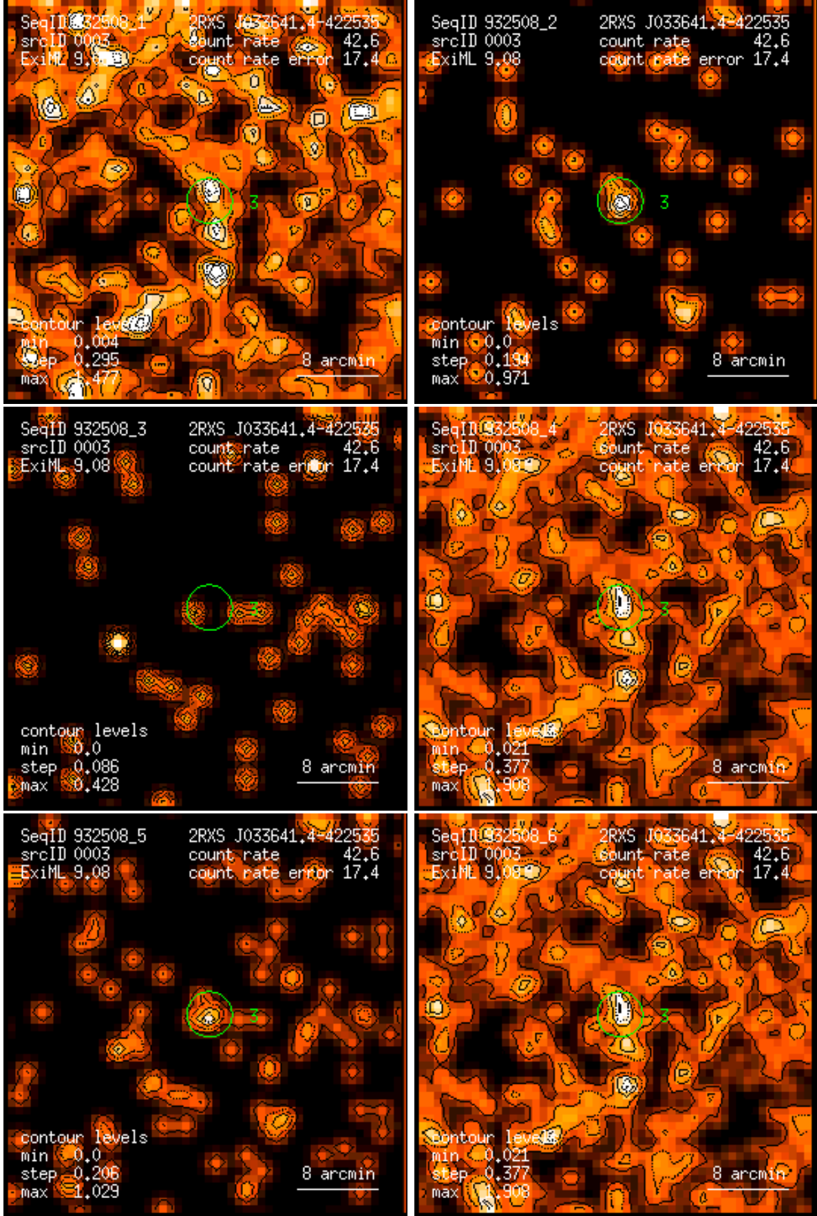
Figure 3: RASS 932508: detection 0003: band rate images, Gaussian filter: (1) PSPC channels 11 – 41, (2) 52 – 90, (3) 91 – 201, (4) 11 – 235, (5) 52 – 201, (6) 11 – 201. Broad band rates in counts/ks. Band rate contour levels in counts/ks/arcmin 2 .
