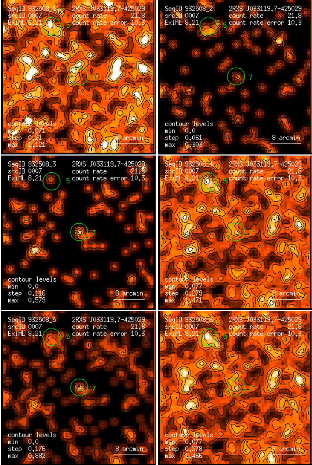
Figure 7: RASS 932508: detection 0007: band rate images, Gaussian filter: (1) PSPC channels 11 – 41, (2) 52 – 90, (3) 91 – 201, (4) 11 – 235, (5) 52 – 201, (6) 11 – 201. Broad band rates in counts/ks. Band rate contour levels in counts/ks/arcmin 2 .
