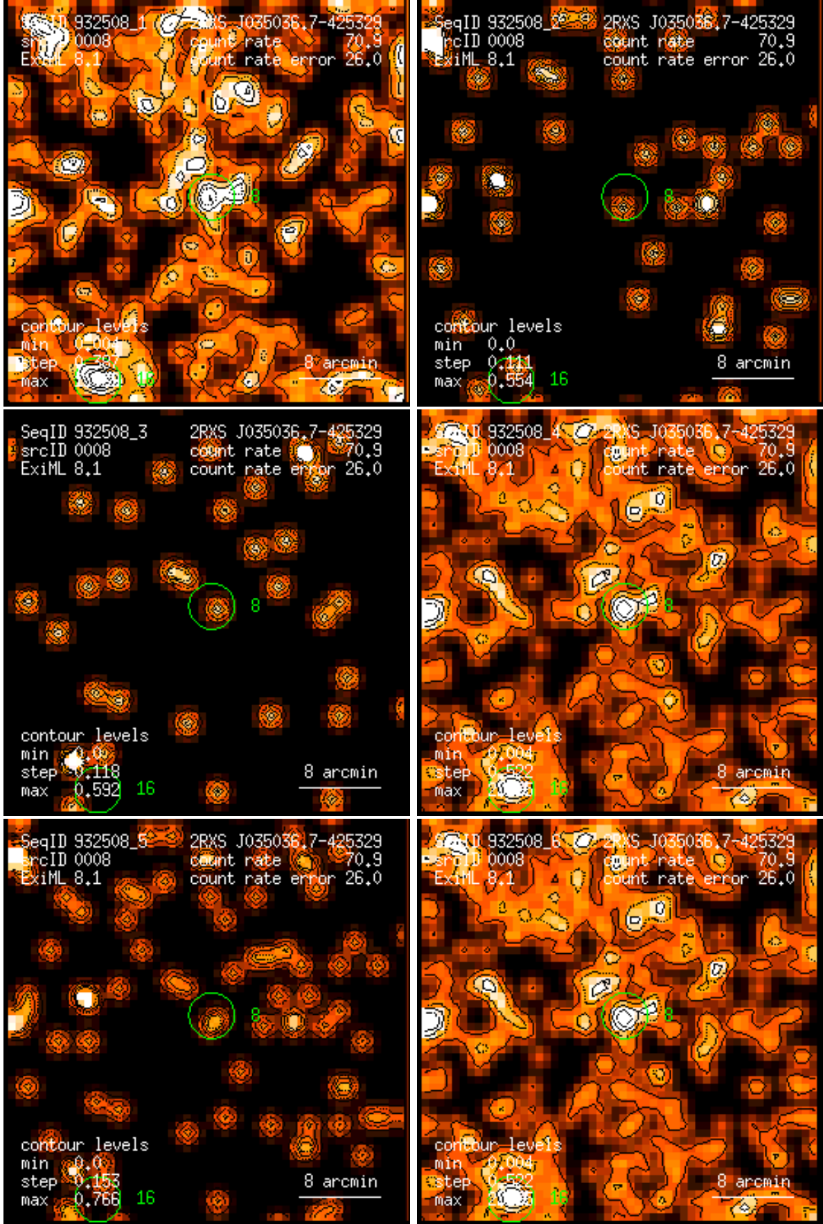
Figure 8: RASS 932508: detection 0008: band rate images, Gaussian filter: (1) PSPC channels 11 – 41, (2) 52 – 90, (3) 91 – 201, (4) 11 – 235, (5) 52 – 201, (6) 11 – 201. Broad band rates in counts/ks. Band rate contour levels in counts/ks/arcmin 2 .
