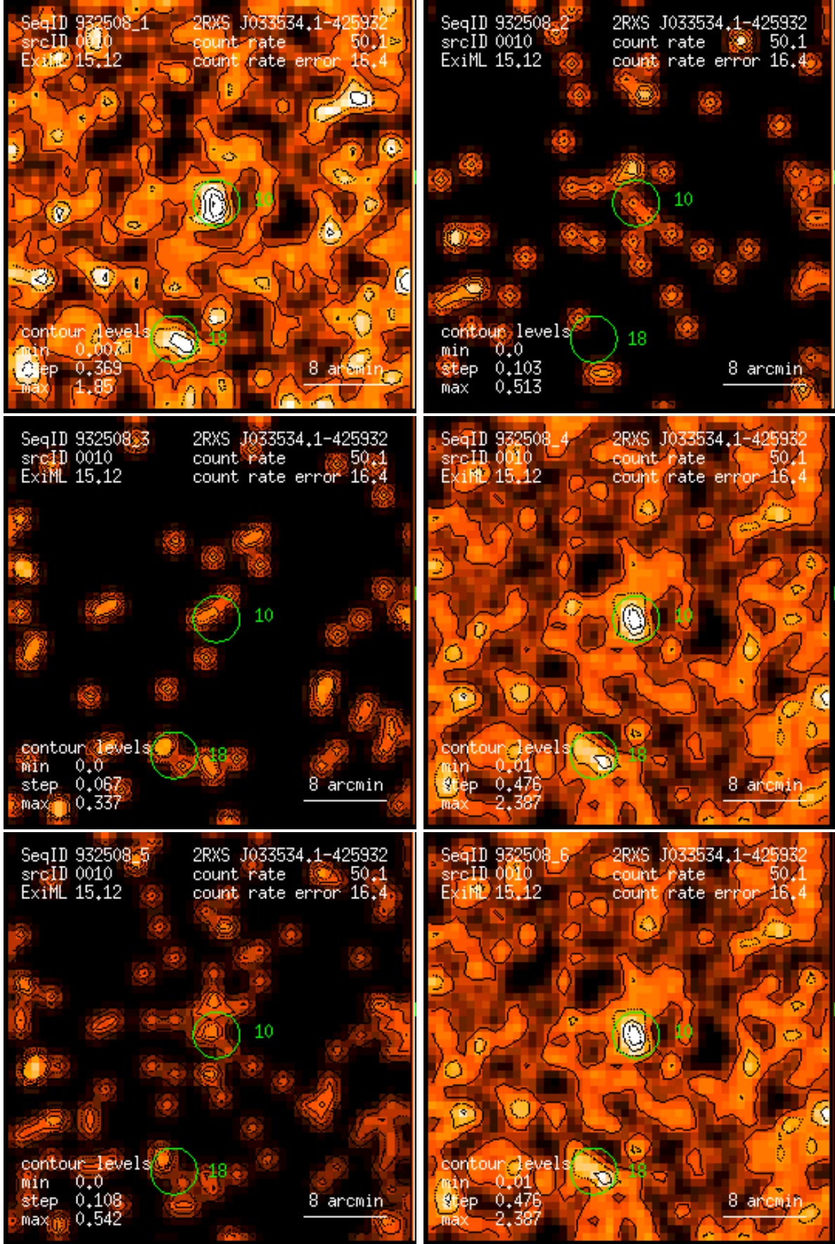
Figure 10: RASS 932508: detection 0010: band rate images, Gaussian filter: (1) PSPC channels 11 – 41, (2) 52 – 90, (3) 91 – 201, (4) 11 – 235, (5) 52 – 201, (6) 11 – 201. Broad band rates in counts/ks. Band rate contour levels in counts/ks/arcmin 2 .
