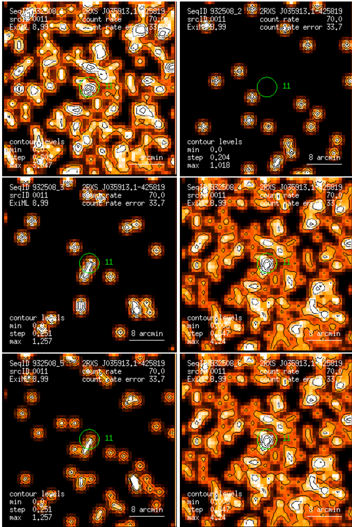
Figure 11: RASS 932508: detection 0011: band rate images, Gaussian filter: (1) PSPC channels 11 – 41, (2) 52 – 90, (3) 91 – 201, (4) 11 – 235, (5) 52 – 201, (6) 11 – 201. Broad band rates in counts/ks. Band rate contour levels in counts/ks/arcmin 2 .
