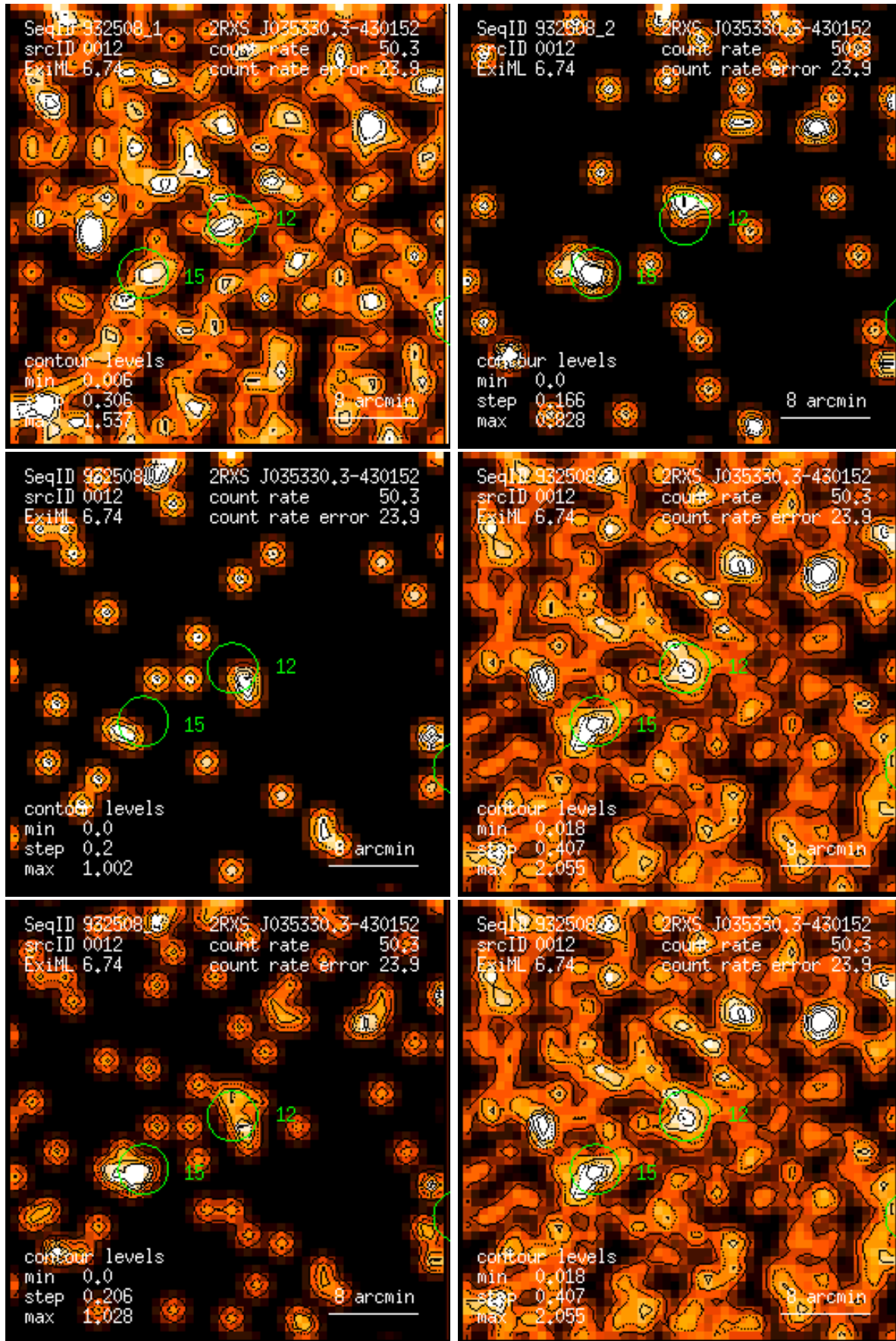
Figure 12: RASS 932508: detection 0012: band rate images, Gaussian filter: (1) PSPC channels 11 – 41, (2) 52 – 90, (3) 91 – 201, (4) 11 – 235, (5) 52 – 201, (6) 11 – 201. Broad band rates in counts/ks. Band rate contour levels in counts/ks/arcmin 2 .
