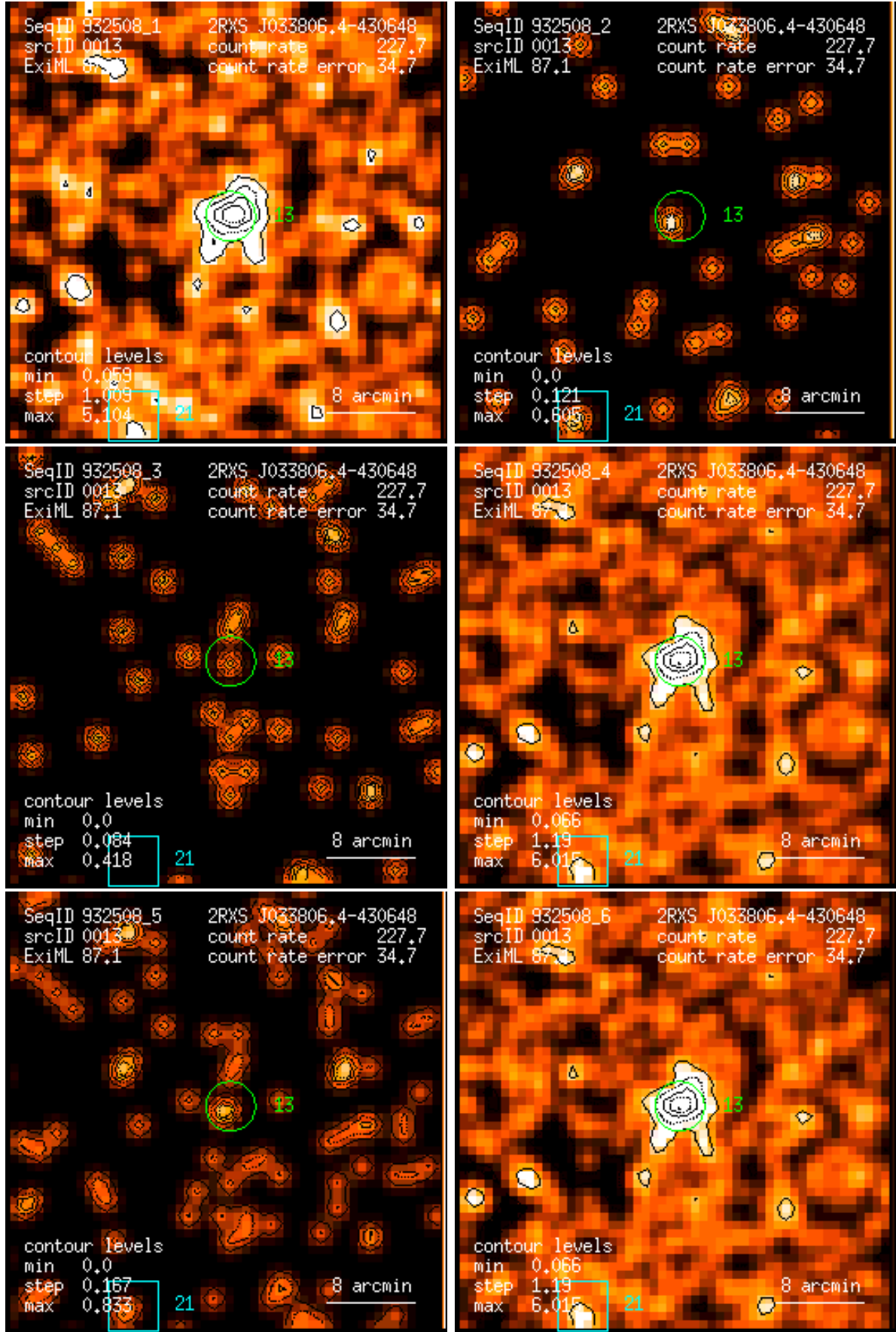
Figure 13: RASS 932508: detection 0013: band rate images, Gaussian filter: (1) PSPC channels 11 – 41, (2) 52 – 90, (3) 91 – 201, (4) 11 – 235, (5) 52 – 201, (6) 11 – 201. Broad band rates in counts/ks. Band rate contour levels in counts/ks/arcmin 2 .
