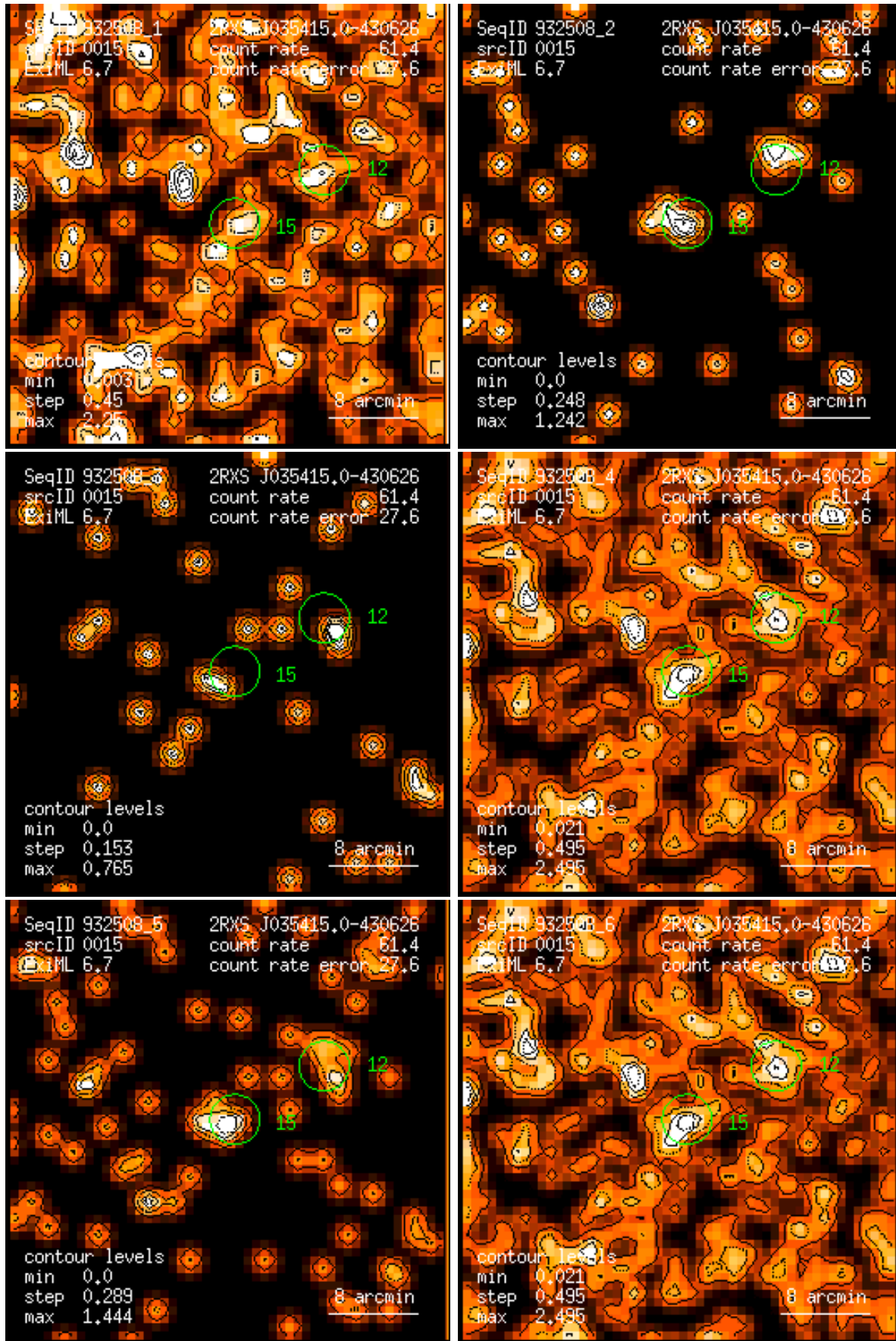
Figure 15: RASS 932508: detection 0015: band rate images, Gaussian filter: (1) PSPC channels 11 – 41, (2) 52 – 90, (3) 91 – 201, (4) 11 – 235, (5) 52 – 201, (6) 11 – 201. Broad band rates in counts/ks. Band rate contour levels in counts/ks/arcmin 2 .
