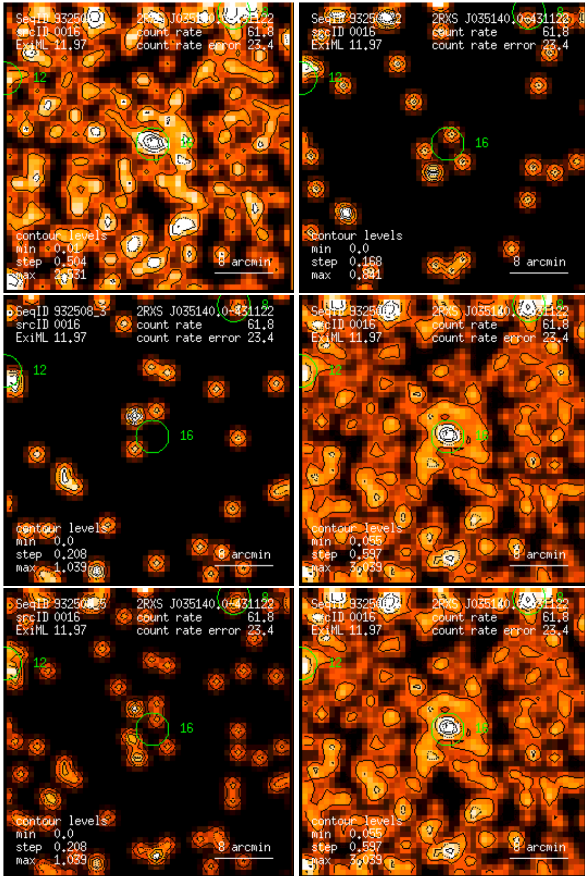
Figure 16: RASS 932508: detection 0016: band rate images, Gaussian filter: (1) PSPC channels 11 – 41, (2) 52 – 90, (3) 91 – 201, (4) 11 – 235, (5) 52 – 201, (6) 11 – 201. Broad band rates in counts/ks. Band rate contour levels in counts/ks/arcmin 2 .
