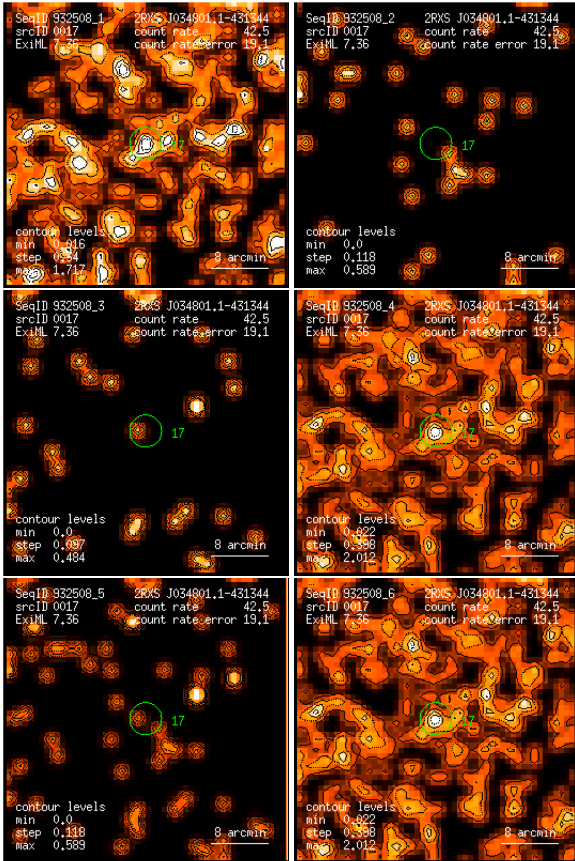
Figure 17: RASS 932508: detection 0017: band rate images, Gaussian filter: (1) PSPC channels 11 – 41, (2) 52 – 90, (3) 91 – 201, (4) 11 – 235, (5) 52 – 201, (6) 11 – 201. Broad band rates in counts/ks. Band rate contour levels in counts/ks/arcmin 2 .
