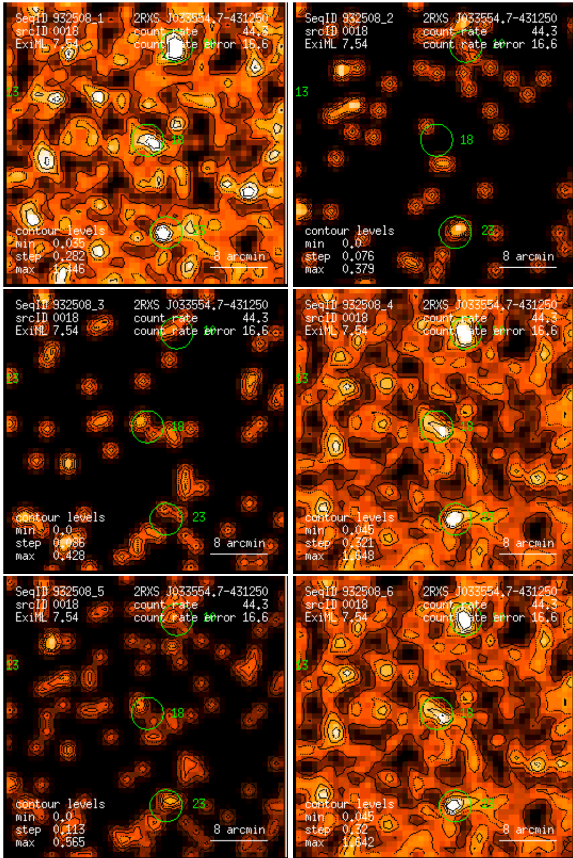
Figure 18: RASS 932508: detection 0018: band rate images, Gaussian filter: (1) PSPC channels 11 – 41, (2) 52 – 90, (3) 91 – 201, (4) 11 – 235, (5) 52 – 201, (6) 11 – 201. Broad band rates in counts/ks. Band rate contour levels in counts/ks/arcmin 2 .
