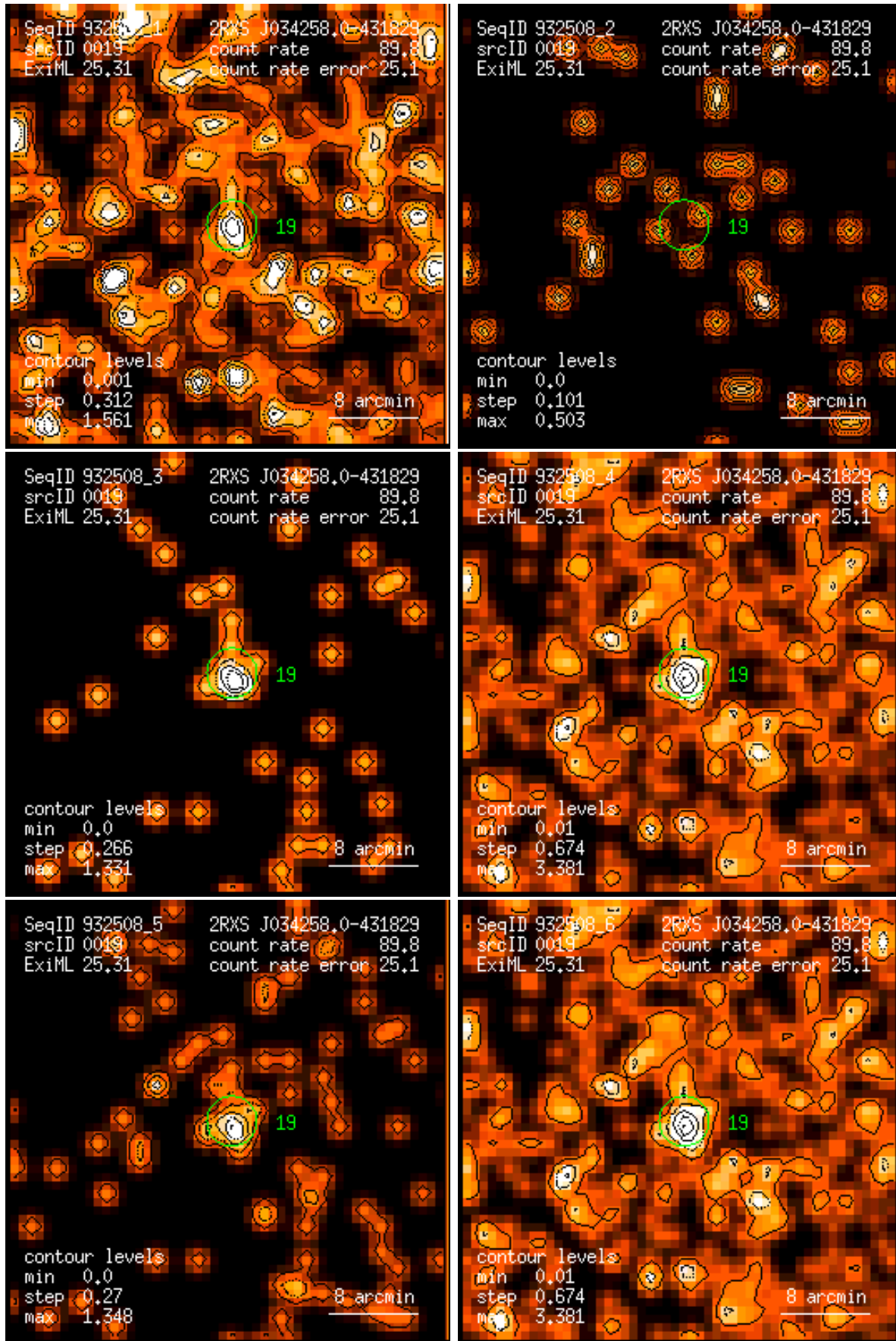
Figure 19: RASS 932508: detection 0019: band rate images, Gaussian filter: (1) PSPC channels 11 – 41, (2) 52 – 90, (3) 91 – 201, (4) 11 – 235, (5) 52 – 201, (6) 11 – 201. Broad band rates in counts/ks. Band rate contour levels in counts/ks/arcmin 2 .
