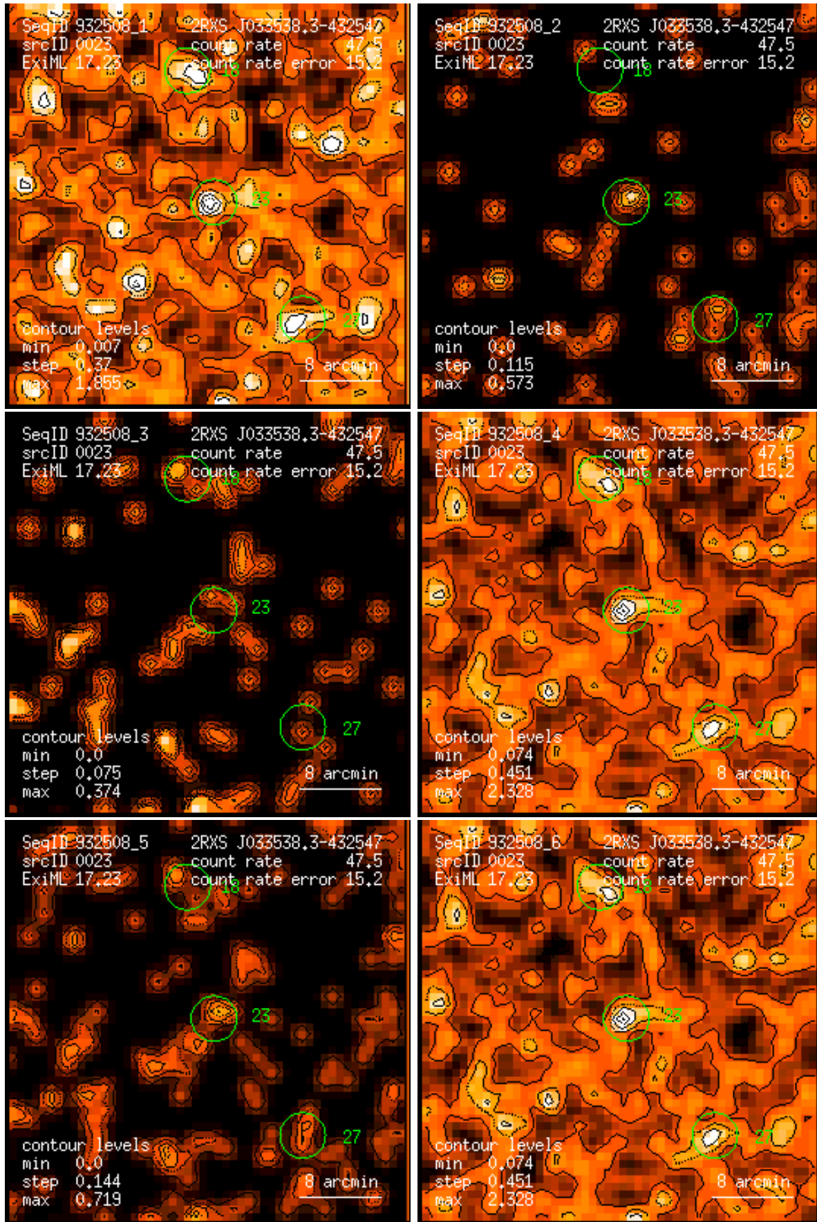
Figure 23: RASS 932508: detection 0023: band rate images, Gaussian filter: (1) PSPC channels 11 – 41, (2) 52 – 90, (3) 91 – 201, (4) 11 – 235, (5) 52 – 201, (6) 11 – 201. Broad band rates in counts/ks. Band rate contour levels in counts/ks/arcmin 2 .
