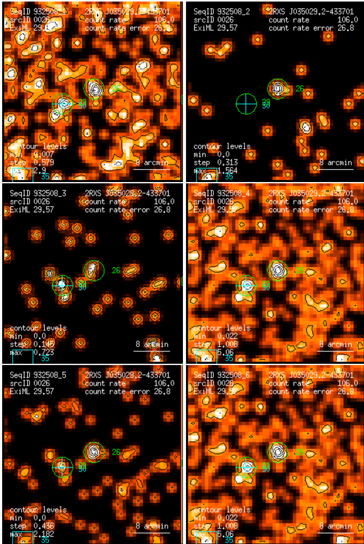
Figure 26: RASS 932508: detection 0026: band rate images, Gaussian filter: (1) PSPC channels 11 – 41, (2) 52 – 90, (3) 91 – 201, (4) 11 – 235, (5) 52 – 201, (6) 11 – 201. Broad band rates in counts/ks. Band rate contour levels in counts/ks/arcmin 2 .
