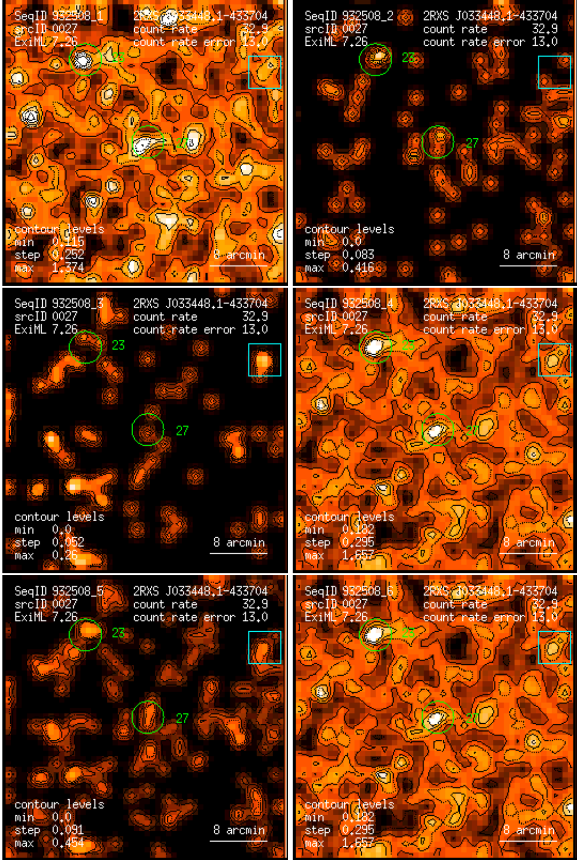
Figure 27: RASS 932508: detection 0027: band rate images, Gaussian filter: (1) PSPC channels 11 – 41, (2) 52 – 90, (3) 91 – 201, (4) 11 – 235, (5) 52 – 201, (6) 11 – 201. Broad band rates in counts/ks. Band rate contour levels in counts/ks/arcmin 2 .
