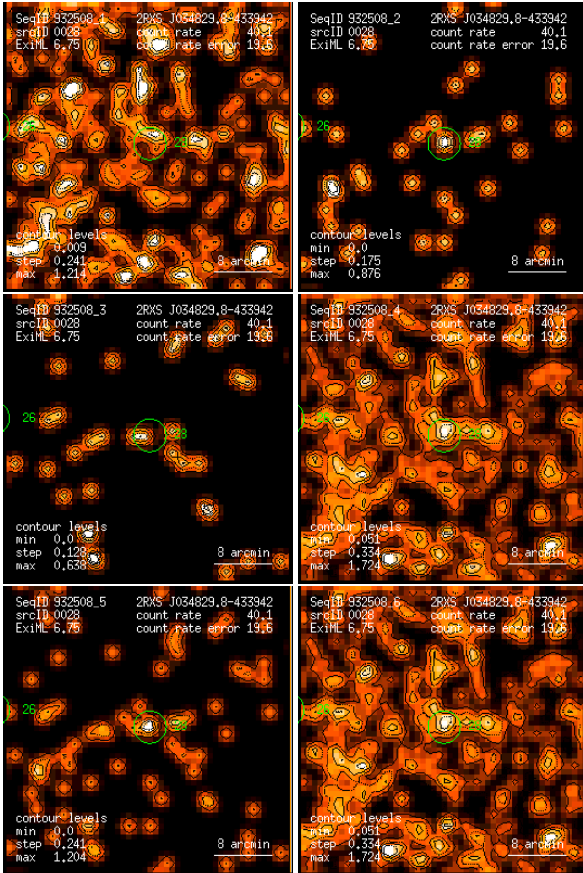
Figure 28: RASS 932508: detection 0028: band rate images, Gaussian filter: (1) PSPC channels 11 – 41, (2) 52 – 90, (3) 91 – 201, (4) 11 – 235, (5) 52 – 201, (6) 11 – 201. Broad band rates in counts/ks. Band rate contour levels in counts/ks/arcmin 2 .
