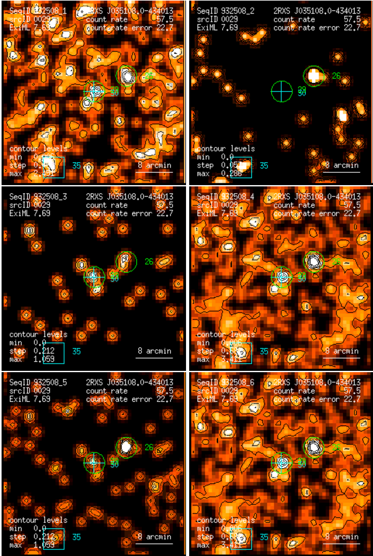
Figure 29: RASS 932508: detection 0029: band rate images, Gaussian filter: (1) PSPC channels 11 – 41, (2) 52 – 90, (3) 91 – 201, (4) 11 – 235, (5) 52 – 201, (6) 11 – 201. Broad band rates in counts/ks. Band rate contour levels in counts/ks/arcmin 2 .
