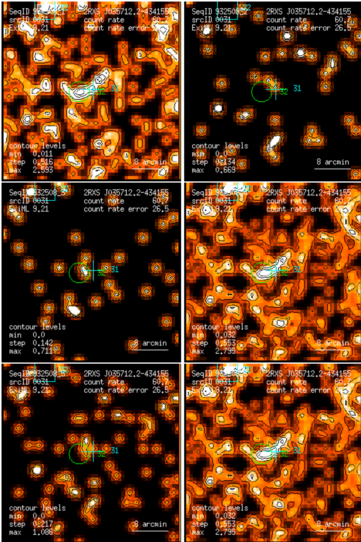
Figure 31: RASS 932508: detection 0031: band rate images, Gaussian filter: (1) PSPC channels 11 – 41, (2) 52 – 90, (3) 91 – 201, (4) 11 – 235, (5) 52 – 201, (6) 11 – 201. Broad band rates in counts/ks. Band rate contour levels in counts/ks/arcmin 2 .
