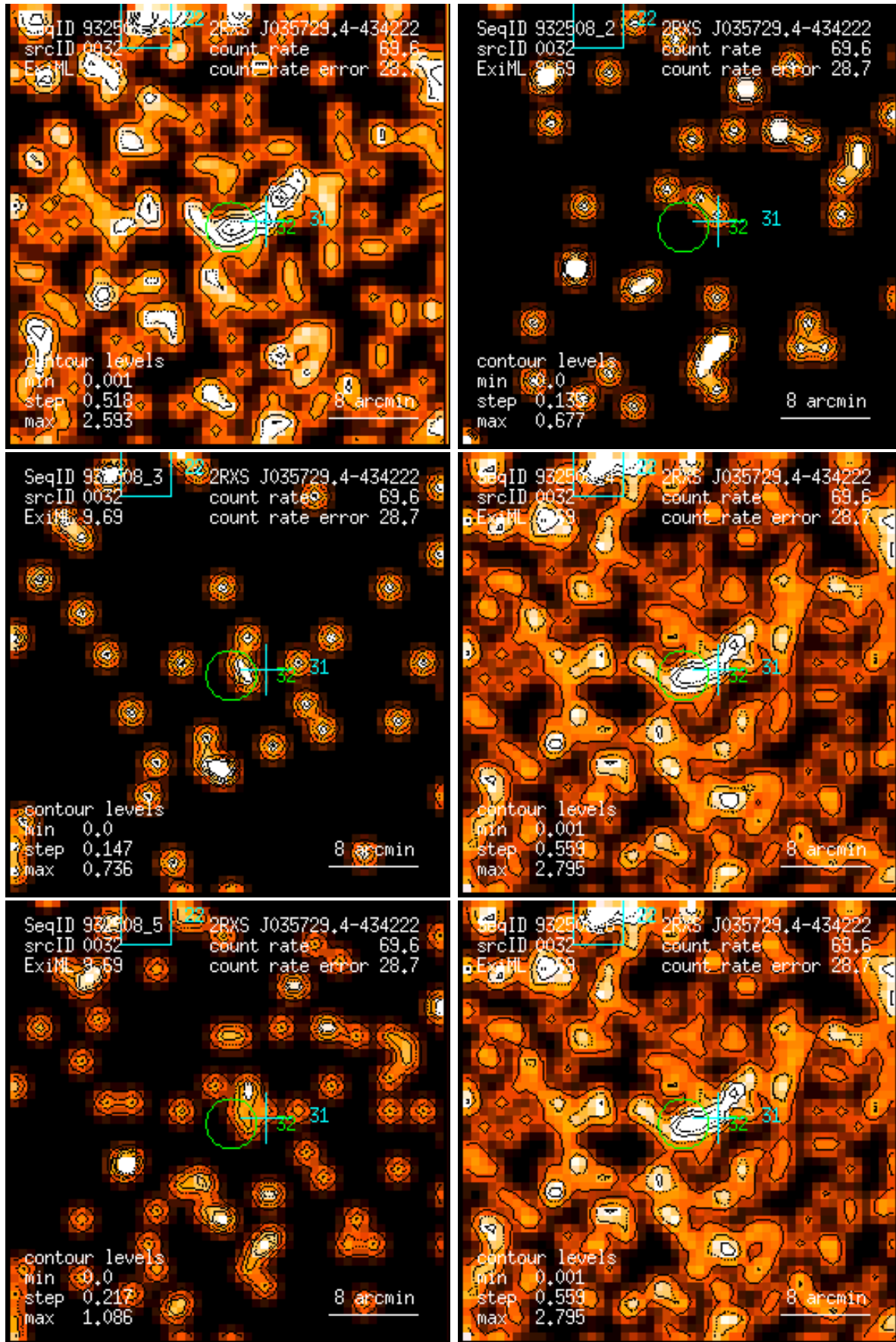
Figure 32: RASS 932508: detection 0032: band rate images, Gaussian filter: (1) PSPC channels 11 – 41, (2) 52 – 90, (3) 91 – 201, (4) 11 – 235, (5) 52 – 201, (6) 11 – 201. Broad band rates in counts/ks. Band rate contour levels in counts/ks/arcmin 2 .
