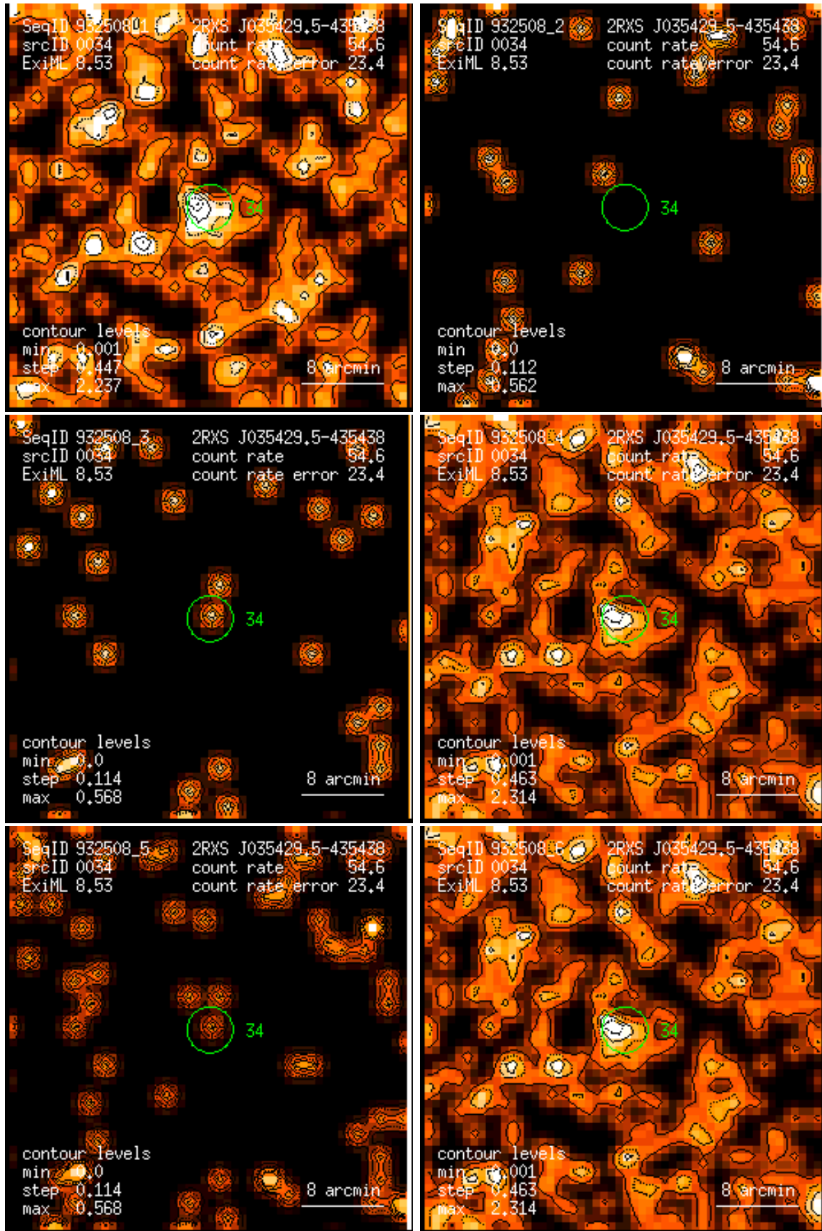
Figure 34: RASS 932508: detection 0034: band rate images, Gaussian filter: (1) PSPC channels 11 – 41, (2) 52 – 90, (3) 91 – 201, (4) 11 – 235, (5) 52 – 201, (6) 11 – 201. Broad band rates in counts/ks. Band rate contour levels in counts/ks/arcmin 2 .
