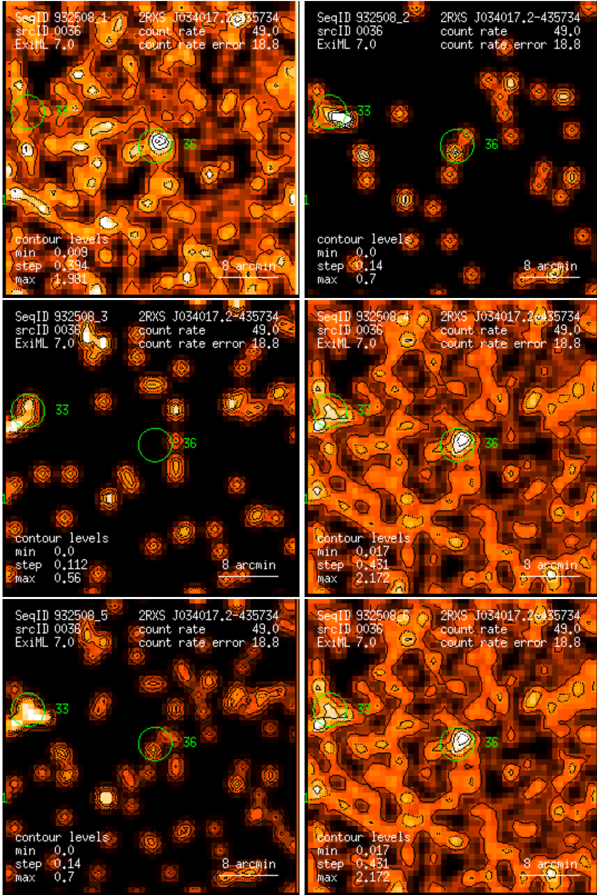
Figure 36: RASS 932508: detection 0036: band rate images, Gaussian filter: (1) PSPC channels 11 – 41, (2) 52 – 90, (3) 91 – 201, (4) 11 – 235, (5) 52 – 201, (6) 11 – 201. Broad band rates in counts/ks. Band rate contour levels in counts/ks/arcmin 2 .
