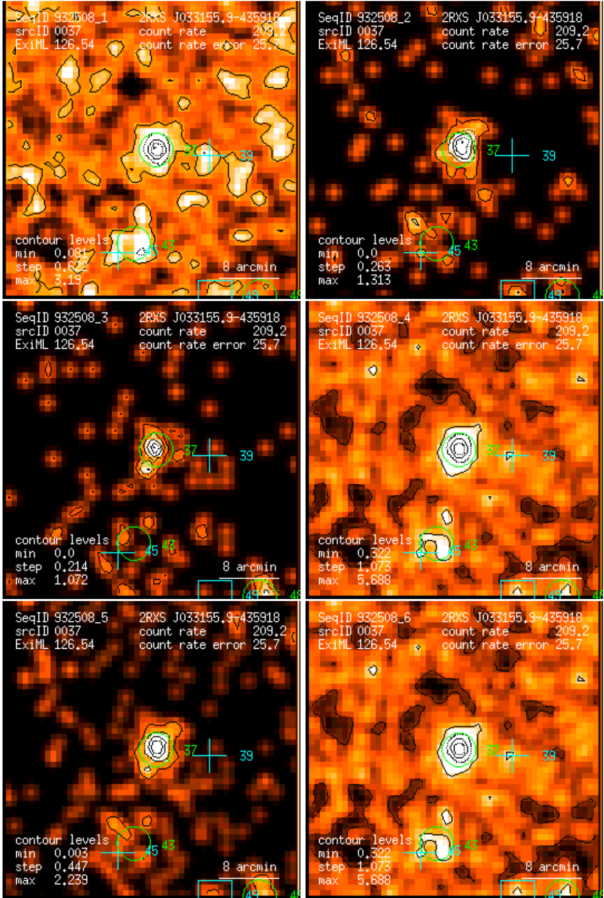
Figure 37: RASS 932508: detection 0037: band rate images, Gaussian filter: (1) PSPC channels 11 – 41, (2) 52 – 90, (3) 91 – 201, (4) 11 – 235, (5) 52 – 201, (6) 11 – 201. Broad band rates in counts/ks. Band rate contour levels in counts/ks/arcmin 2 .
