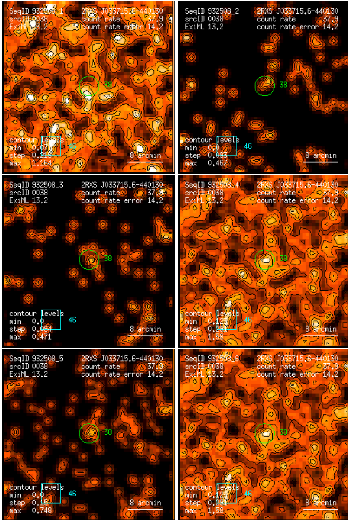
Figure 38: RASS 932508: detection 0038: band rate images, Gaussian filter: (1) PSPC channels 11 – 41, (2) 52 – 90, (3) 91 – 201, (4) 11 – 235, (5) 52 – 201, (6) 11 – 201. Broad band rates in counts/ks. Band rate contour levels in counts/ks/arcmin 2 .
