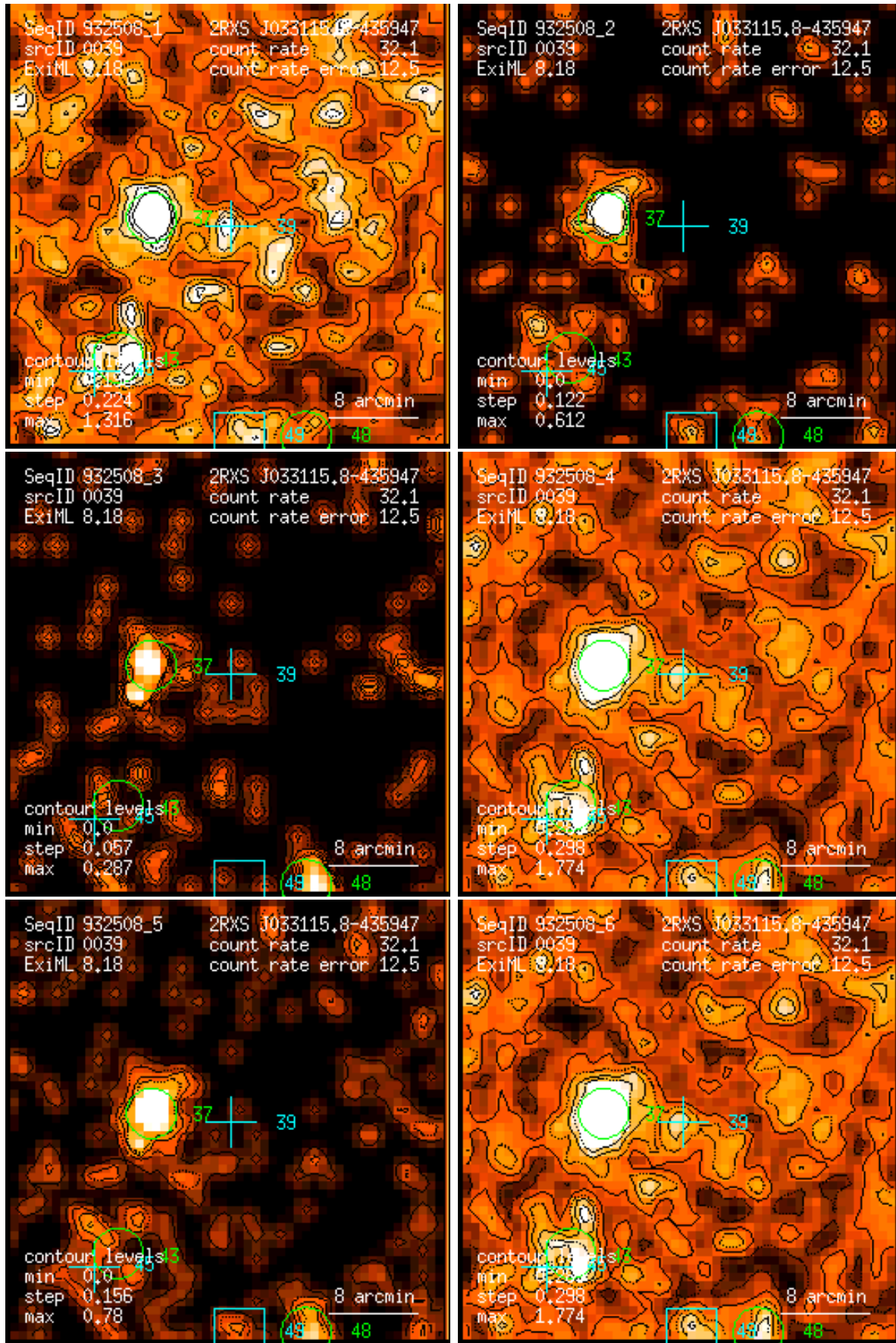
Figure 39: RASS 932508: detection 0039: band rate images, Gaussian filter: (1) PSPC channels 11 – 41, (2) 52 – 90, (3) 91 – 201, (4) 11 – 235, (5) 52 – 201, (6) 11 – 201. Broad band rates in counts/ks. Band rate contour levels in counts/ks/arcmin 2 .
