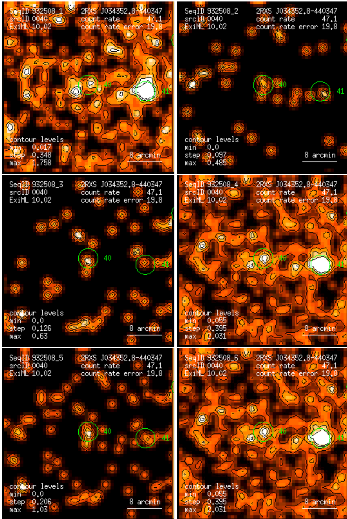
Figure 40: RASS 932508: detection 0040: band rate images, Gaussian filter: (1) PSPC channels 11 – 41, (2) 52 – 90, (3) 91 – 201, (4) 11 – 235, (5) 52 – 201, (6) 11 – 201. Broad band rates in counts/ks. Band rate contour levels in counts/ks/arcmin 2 .
