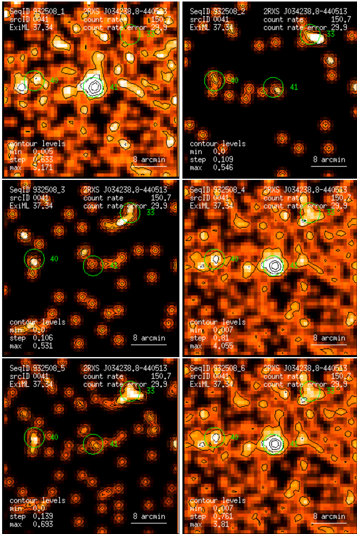
Figure 41: RASS 932508: detection 0041: band rate images, Gaussian filter: (1) PSPC channels 11 – 41, (2) 52 – 90, (3) 91 – 201, (4) 11 – 235, (5) 52 – 201, (6) 11 – 201. Broad band rates in counts/ks. Band rate contour levels in counts/ks/arcmin 2 .
