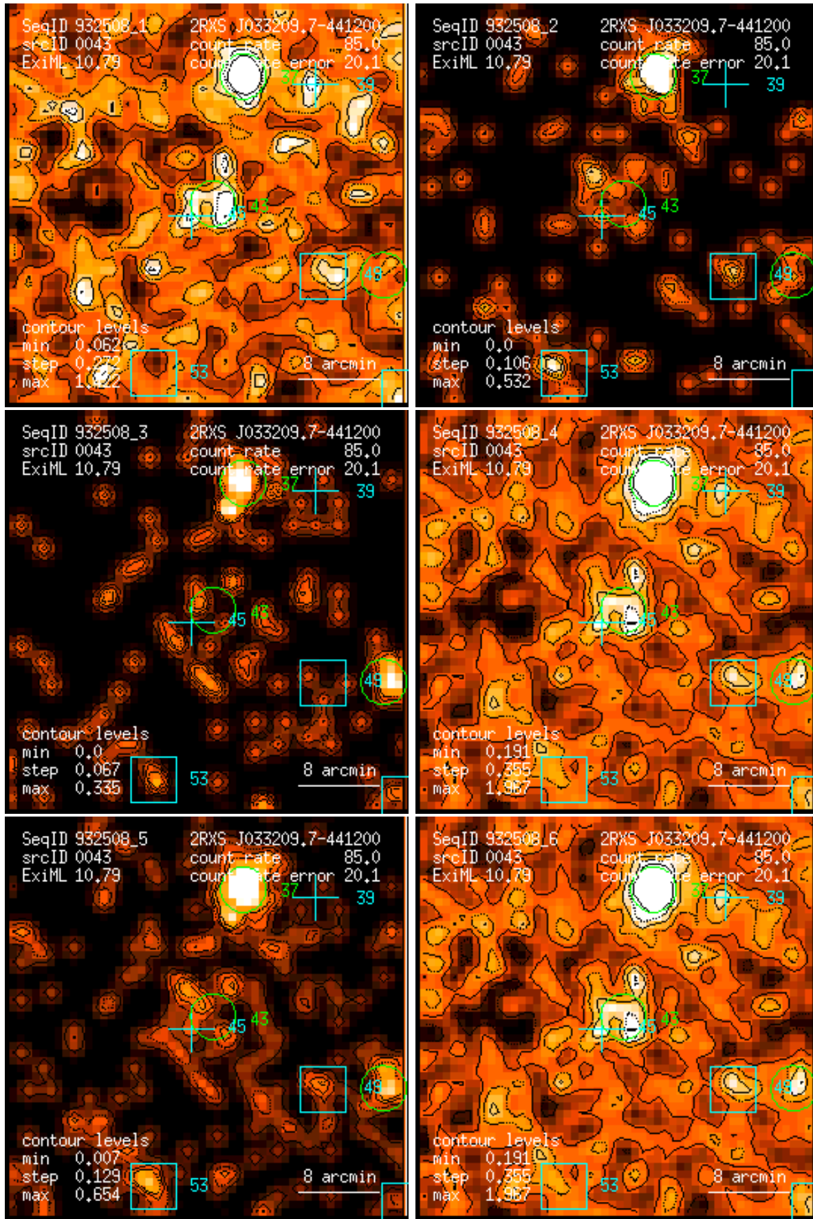
Figure 43: RASS 932508: detection 0043: band rate images, Gaussian filter: (1) PSPC channels 11 – 41, (2) 52 – 90, (3) 91 – 201, (4) 11 – 235, (5) 52 – 201, (6) 11 – 201. Broad band rates in counts/ks. Band rate contour levels in counts/ks/arcmin 2 .
