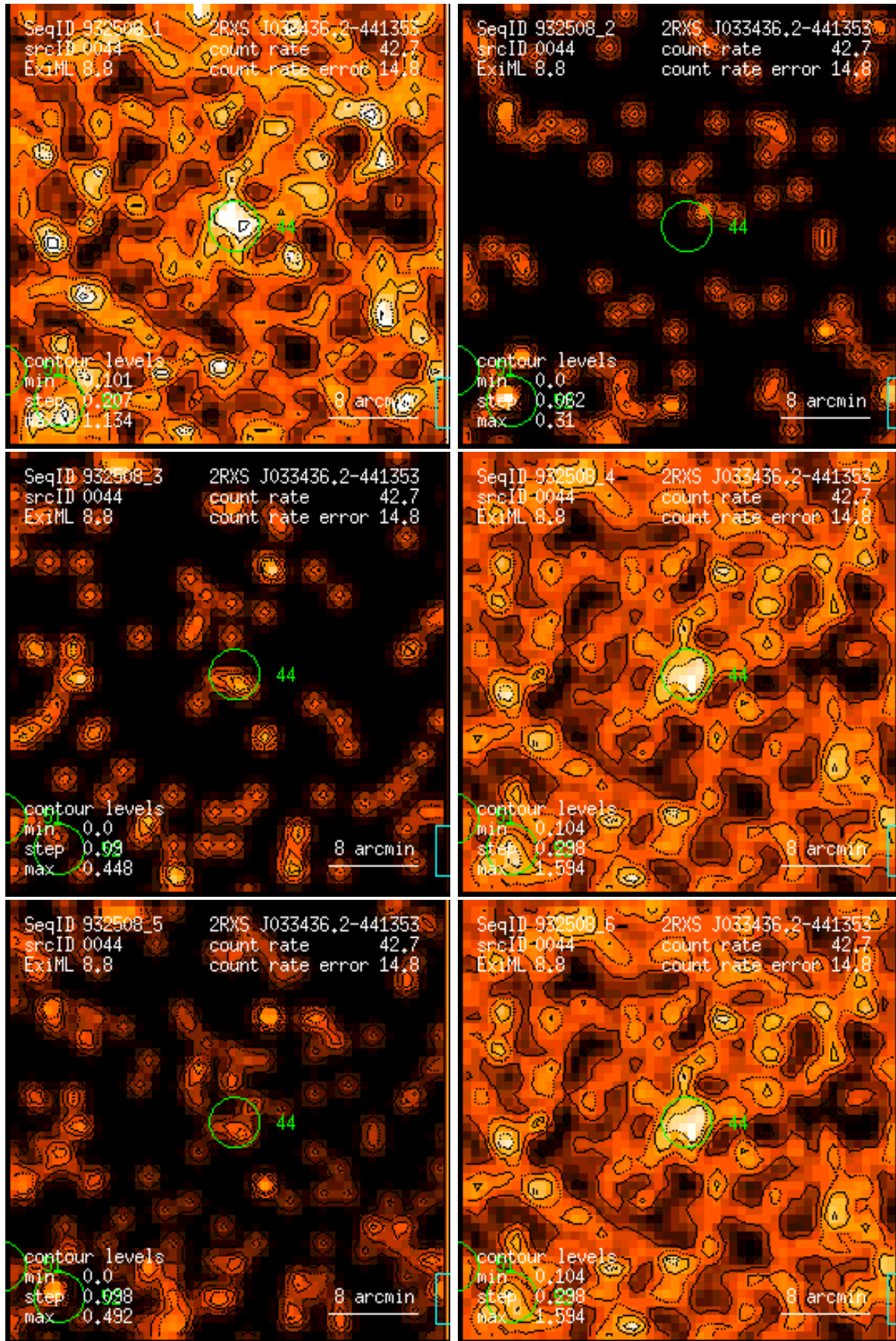
Figure 44: RASS 932508: detection 0044: band rate images, Gaussian filter: (1) PSPC channels 11 – 41, (2) 52 – 90, (3) 91 – 201, (4) 11 – 235, (5) 52 – 201, (6) 11 – 201. Broad band rates in counts/ks. Band rate contour levels in counts/ks/arcmin 2 .
