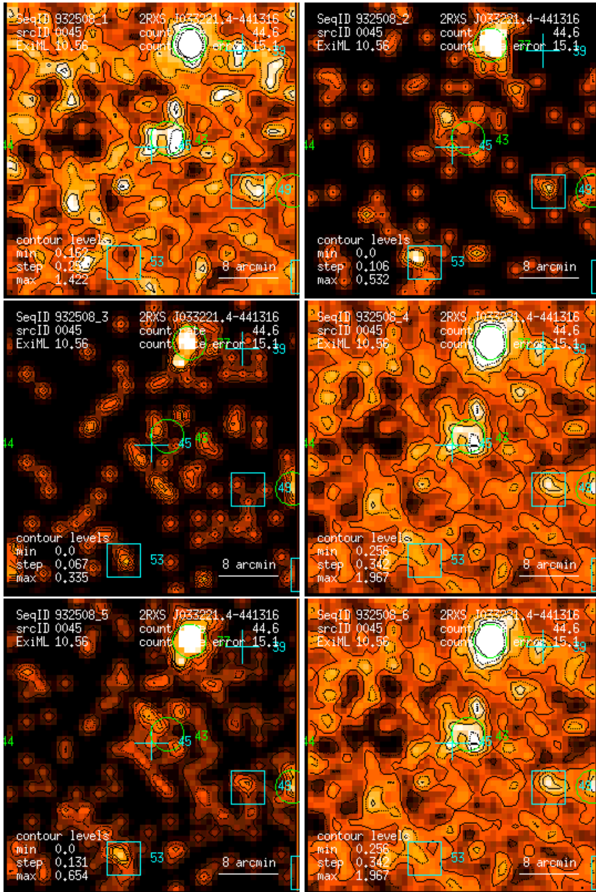
Figure 45: RASS 932508: detection 0045: band rate images, Gaussian filter: (1) PSPC channels 11 – 41, (2) 52 – 90, (3) 91 – 201, (4) 11 – 235, (5) 52 – 201, (6) 11 – 201. Broad band rates in counts/ks. Band rate contour levels in counts/ks/arcmin 2 .
