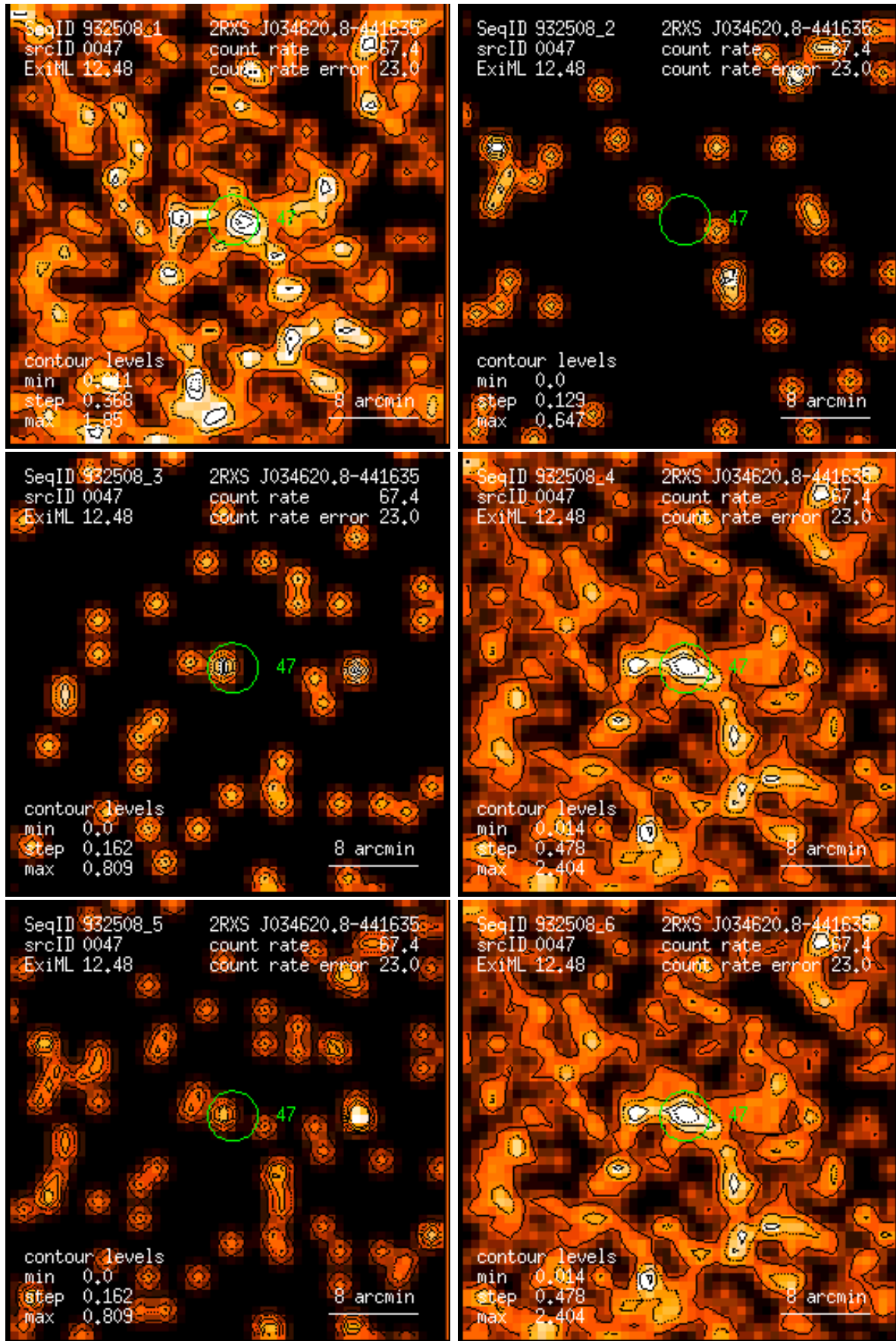
Figure 47: RASS 932508: detection 0047: band rate images, Gaussian filter: (1) PSPC channels 11 – 41, (2) 52 – 90, (3) 91 – 201, (4) 11 – 235, (5) 52 – 201, (6) 11 – 201. Broad band rates in counts/ks. Band rate contour levels in counts/ks/arcmin 2 .
