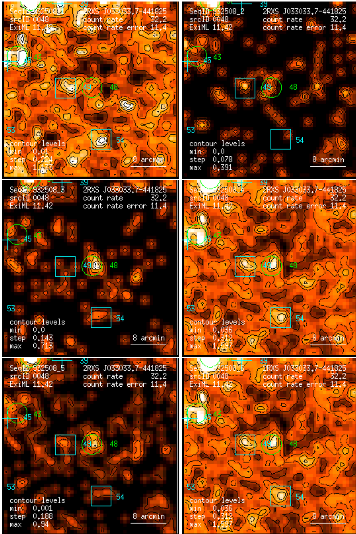
Figure 48: RASS 932508: detection 0048: band rate images, Gaussian filter: (1) PSPC channels 11 – 41, (2) 52 – 90, (3) 91 – 201, (4) 11 – 235, (5) 52 – 201, (6) 11 – 201. Broad band rates in counts/ks. Band rate contour levels in counts/ks/arcmin 2 .
