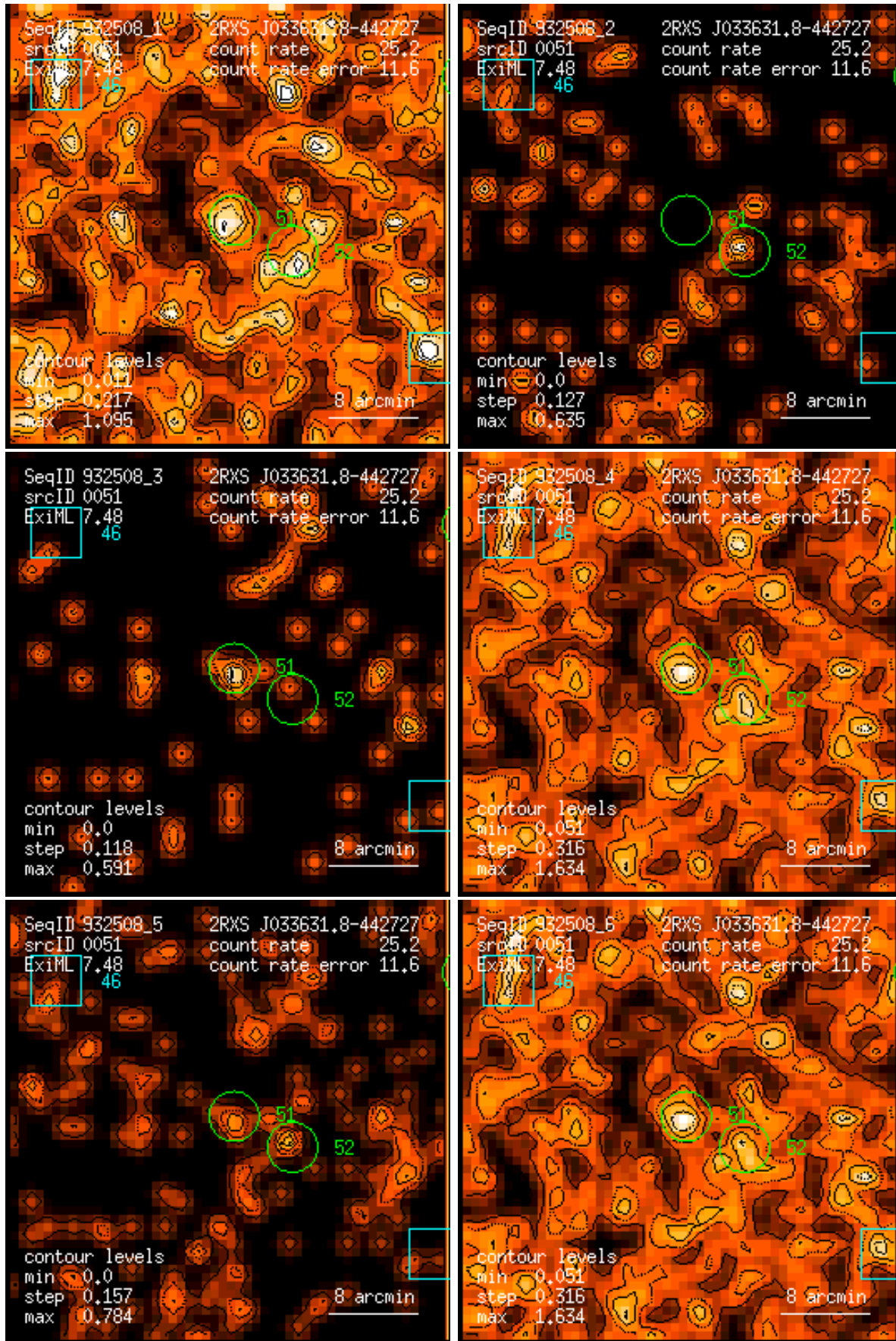
Figure 51: RASS 932508: detection 0051: band rate images, Gaussian filter: (1) PSPC channels 11 – 41, (2) 52 – 90, (3) 91 – 201, (4) 11 – 235, (5) 52 – 201, (6) 11 – 201. Broad band rates in counts/ks. Band rate contour levels in counts/ks/arcmin 2 .
