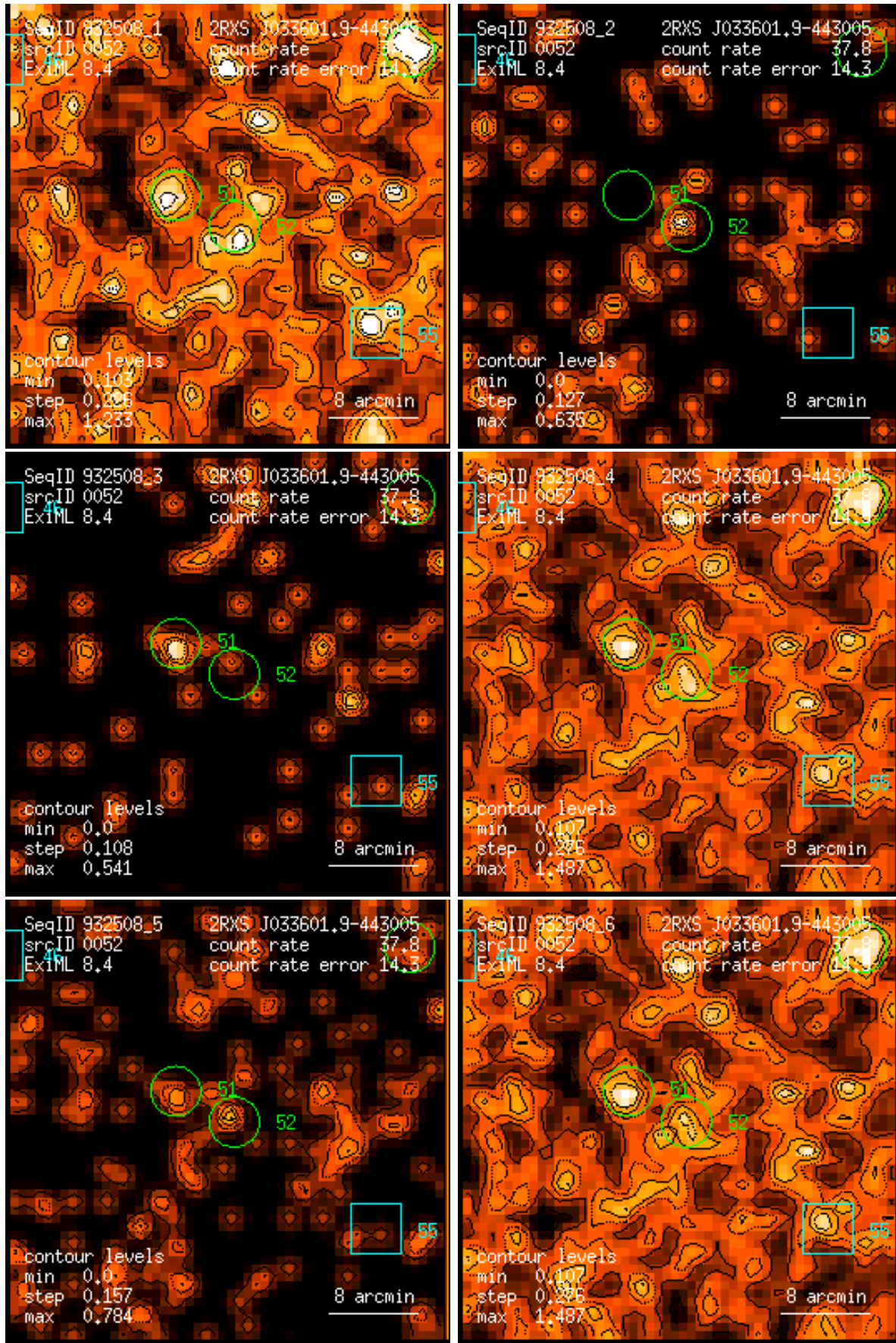
Figure 52: RASS 932508: detection 0052: band rate images, Gaussian filter: (1) PSPC channels 11 – 41, (2) 52 – 90, (3) 91 – 201, (4) 11 – 235, (5) 52 – 201, (6) 11 – 201. Broad band rates in counts/ks. Band rate contour levels in counts/ks/arcmin 2 .
