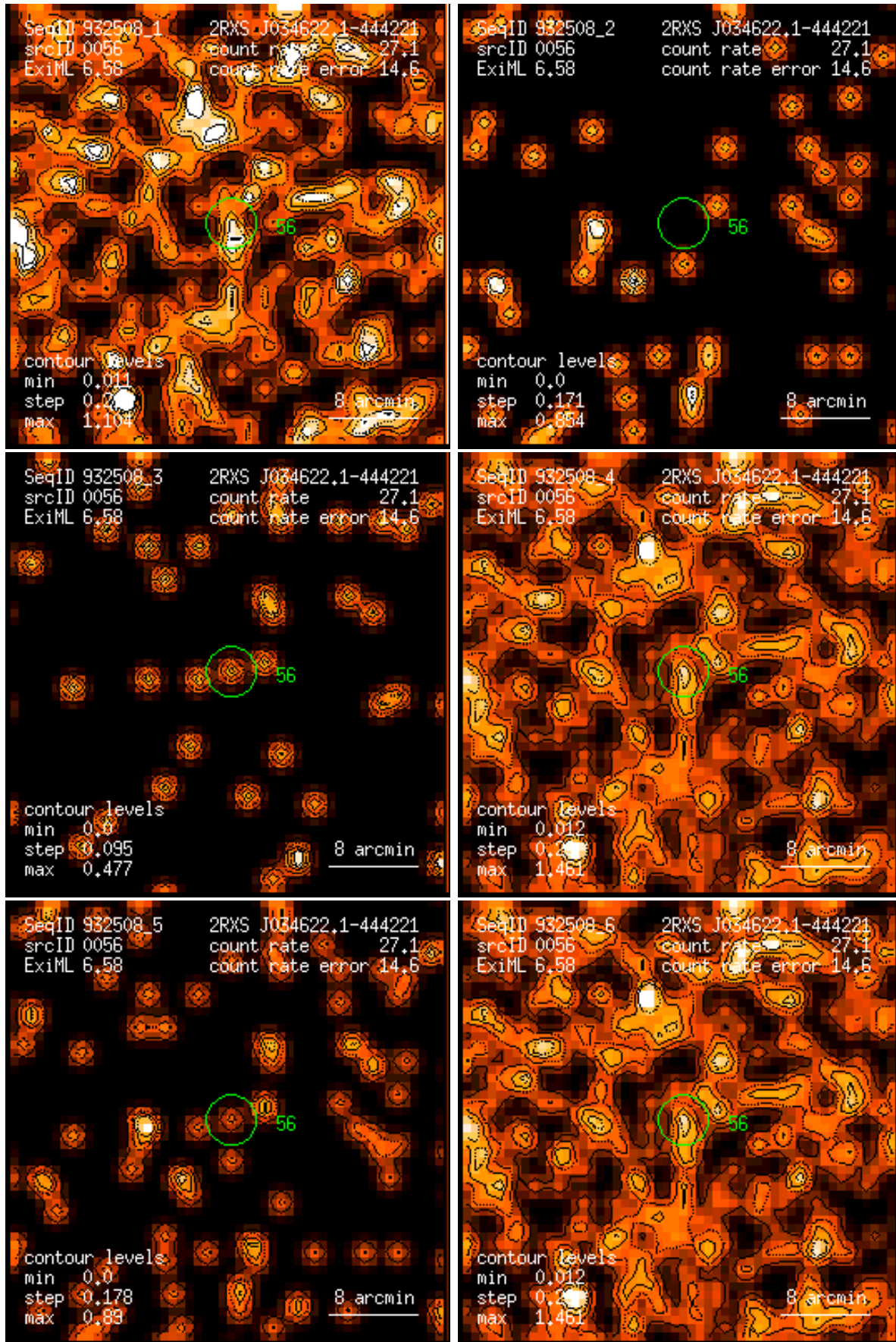
Figure 56: RASS 932508: detection 0056: band rate images, Gaussian filter: (1) PSPC channels 11 – 41, (2) 52 – 90, (3) 91 – 201, (4) 11 – 235, (5) 52 – 201, (6) 11 – 201. Broad band rates in counts/ks. Band rate contour levels in counts/ks/arcmin 2 .
