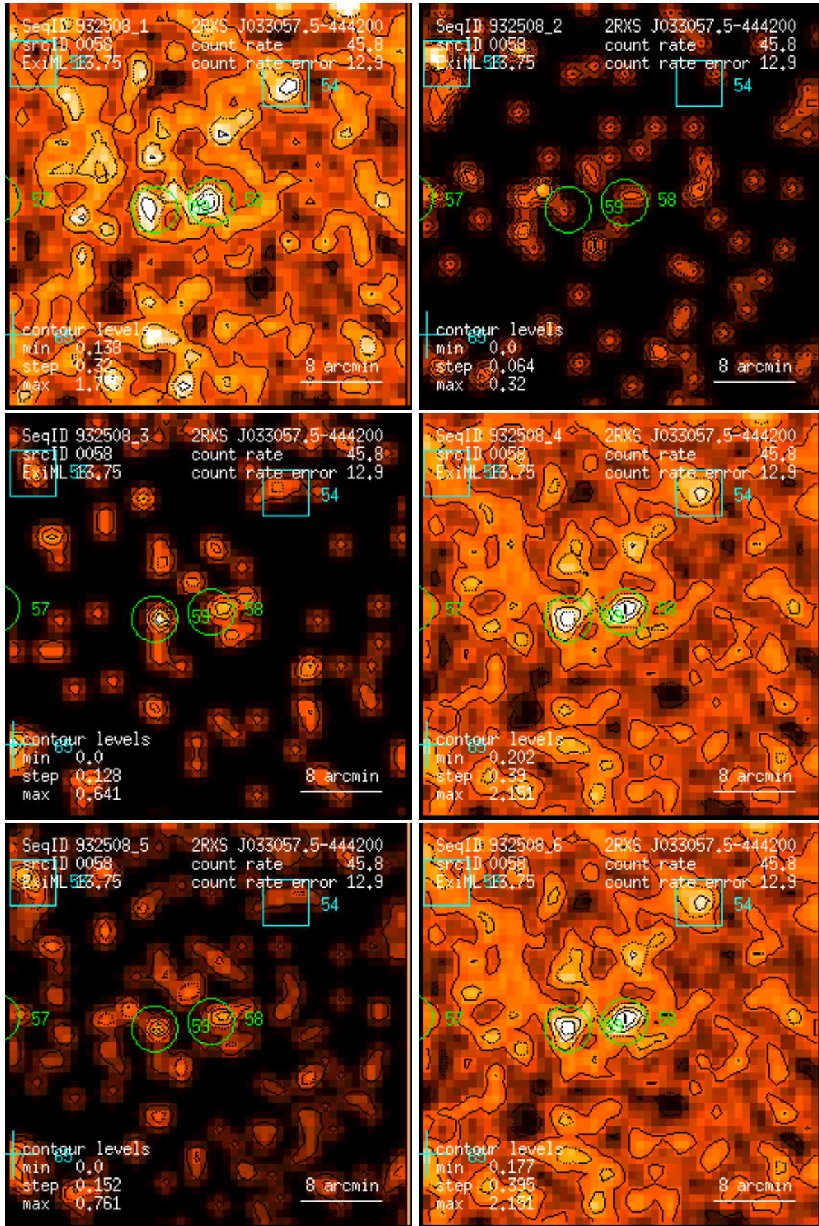
Figure 58: RASS 932508: detection 0058: band rate images, Gaussian filter: (1) PSPC channels 11 – 41, (2) 52 – 90, (3) 91 – 201, (4) 11 – 235, (5) 52 – 201, (6) 11 – 201. Broad band rates in counts/ks. Band rate contour levels in counts/ks/arcmin 2 .
