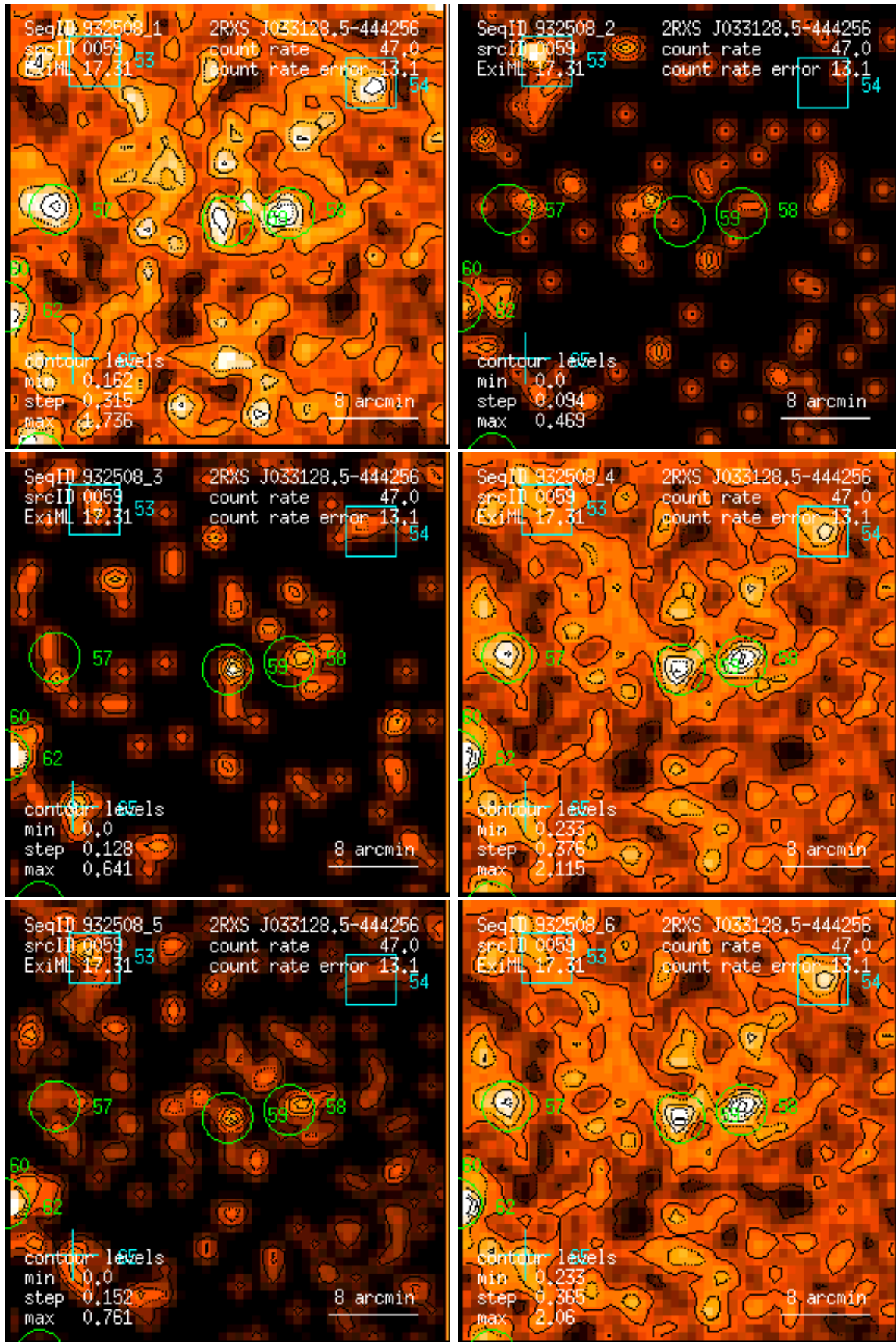
Figure 59: RASS 932508: detection 0059: band rate images, Gaussian filter: (1) PSPC channels 11 – 41, (2) 52 – 90, (3) 91 – 201, (4) 11 – 235, (5) 52 – 201, (6) 11 – 201. Broad band rates in counts/ks. Band rate contour levels in counts/ks/arcmin 2 .
