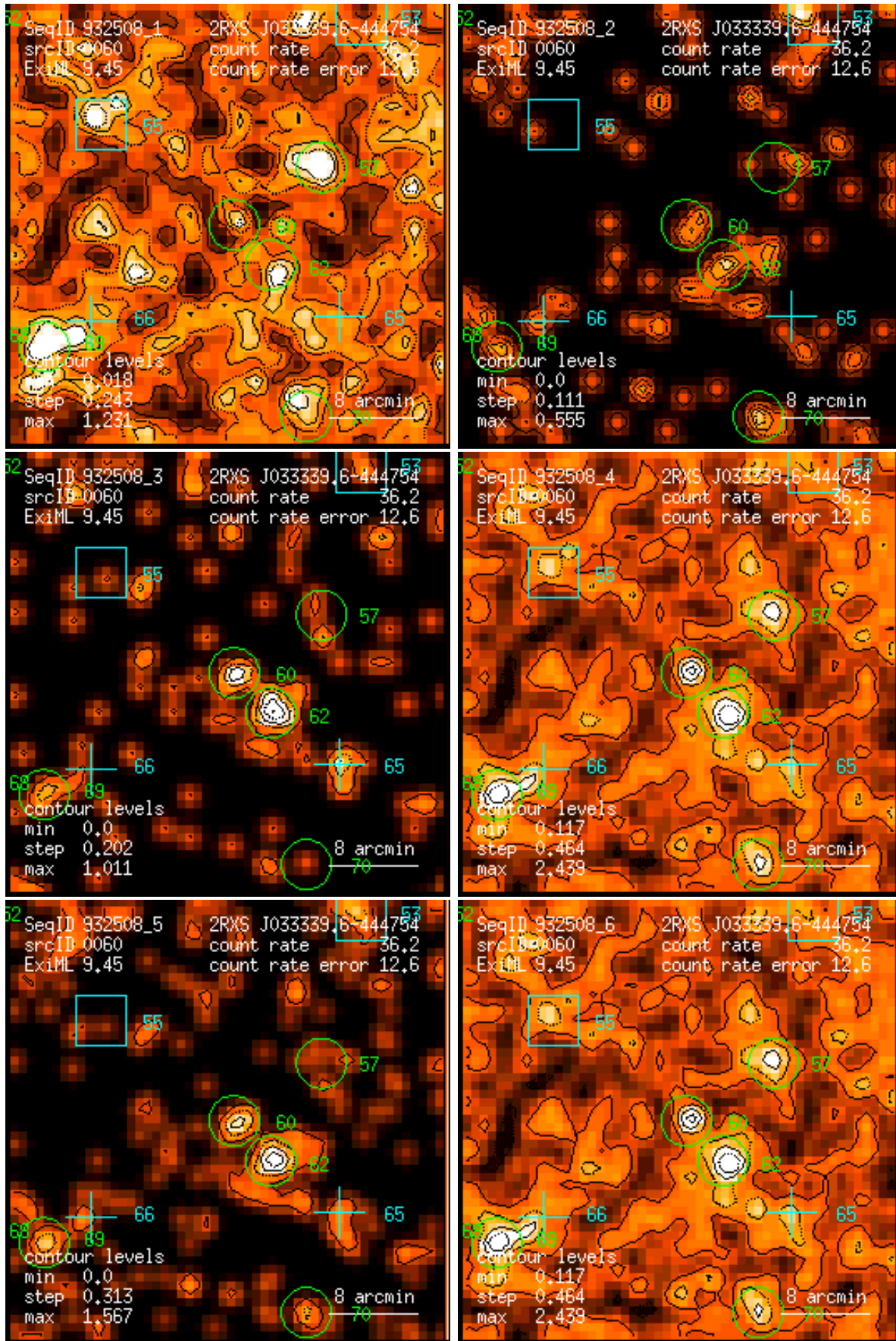
Figure 60: RASS 932508: detection 0060: band rate images, Gaussian filter: (1) PSPC channels 11 – 41, (2) 52 – 90, (3) 91 – 201, (4) 11 – 235, (5) 52 – 201, (6) 11 – 201. Broad band rates in counts/ks. Band rate contour levels in counts/ks/arcmin 2 .
