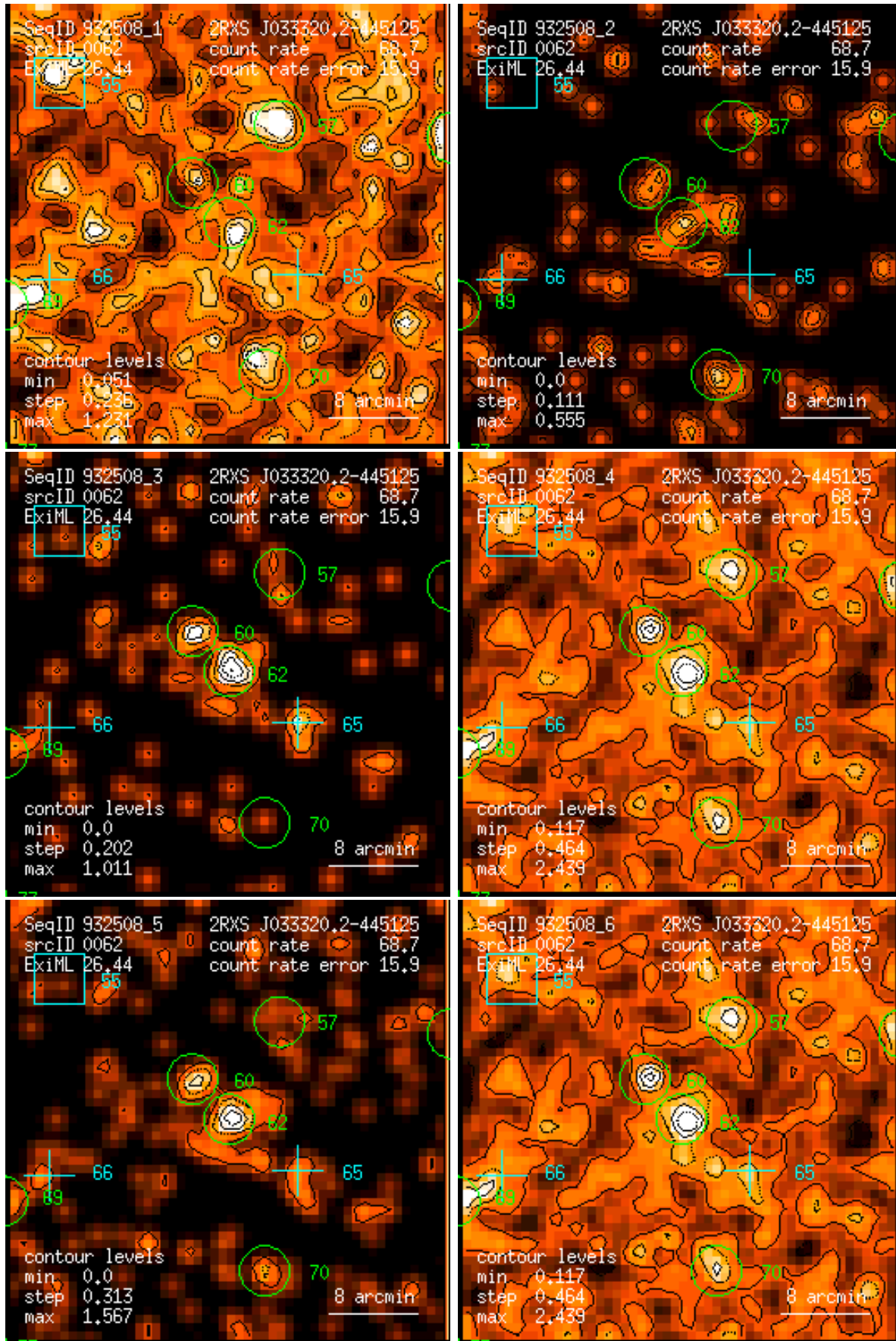
Figure 62: RASS 932508: detection 0062: band rate images, Gaussian filter: (1) PSPC channels 11 – 41, (2) 52 – 90, (3) 91 – 201, (4) 11 – 235, (5) 52 – 201, (6) 11 – 201. Broad band rates in counts/ks. Band rate contour levels in counts/ks/arcmin 2 .
