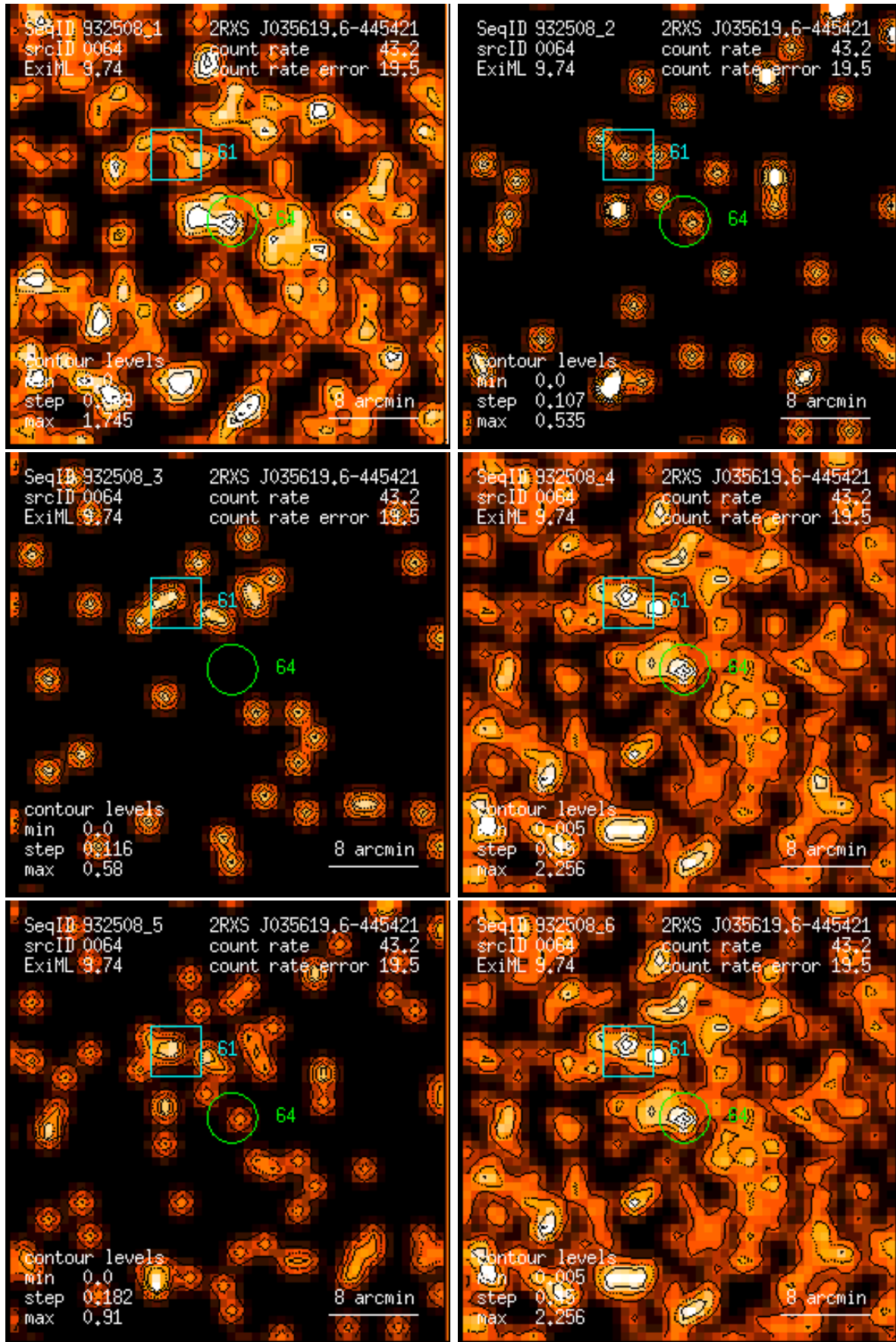
Figure 64: RASS 932508: detection 0064: band rate images, Gaussian filter: (1) PSPC channels 11 – 41, (2) 52 – 90, (3) 91 – 201, (4) 11 – 235, (5) 52 – 201, (6) 11 – 201. Broad band rates in counts/ks. Band rate contour levels in counts/ks/arcmin 2 .
