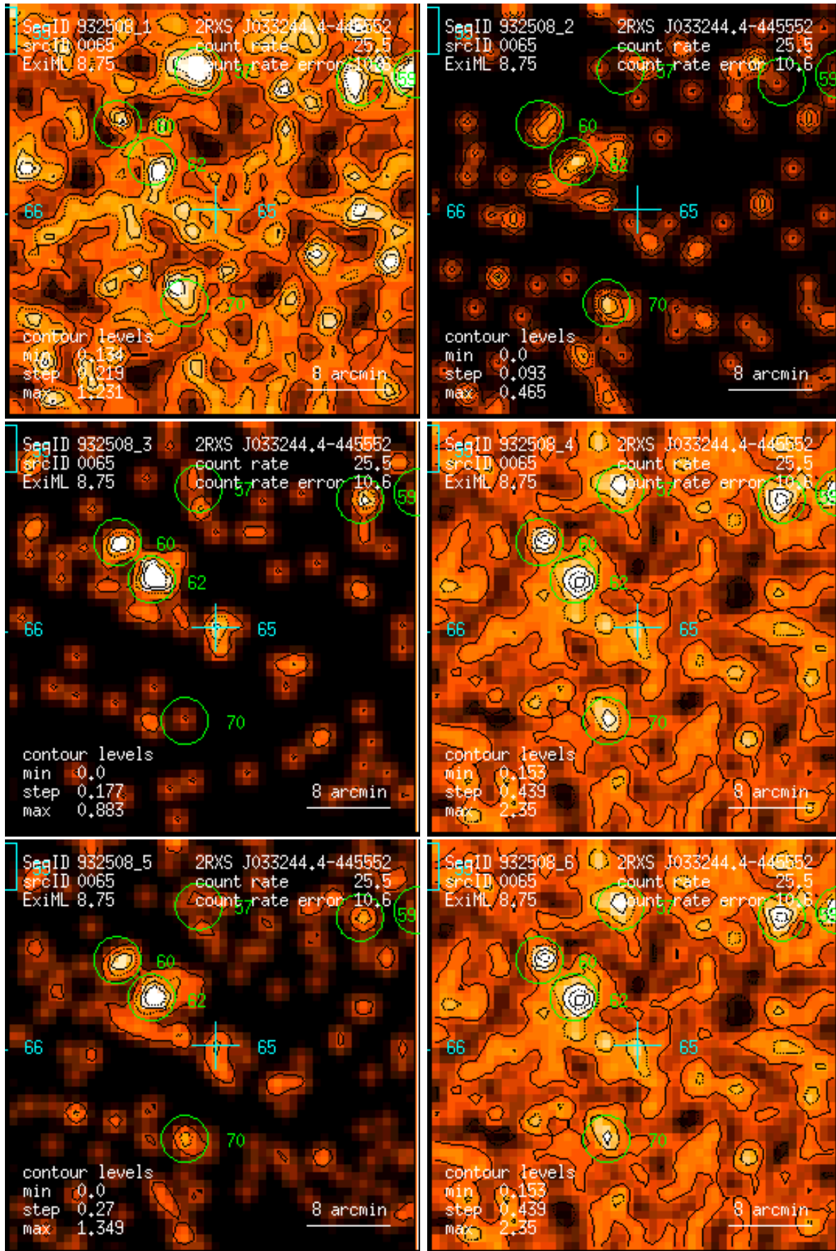
Figure 65: RASS 932508: detection 0065: band rate images, Gaussian filter: (1) PSPC channels 11 – 41, (2) 52 – 90, (3) 91 – 201, (4) 11 – 235, (5) 52 – 201, (6) 11 – 201. Broad band rates in counts/ks. Band rate contour levels in counts/ks/arcmin 2 .
