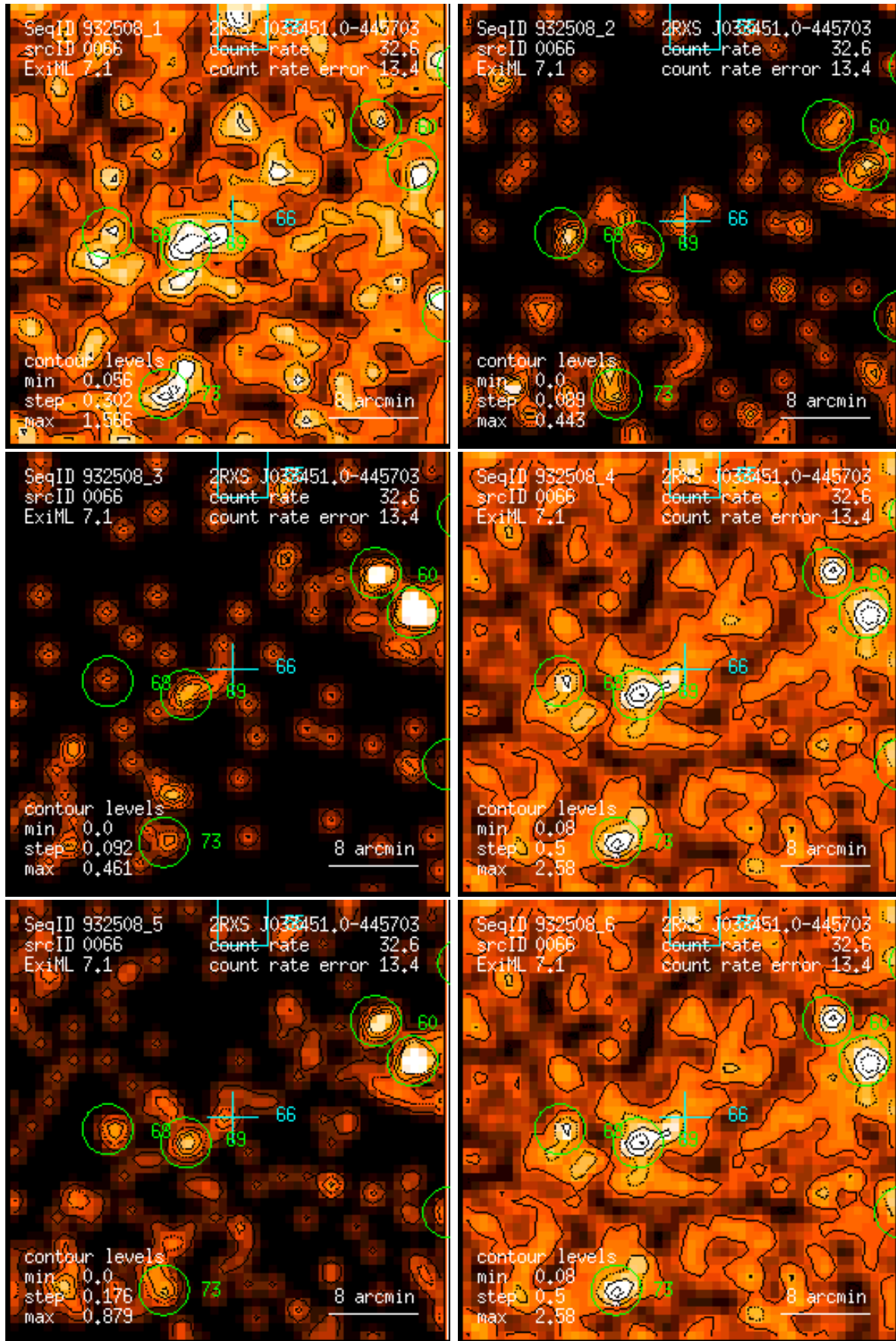
Figure 66: RASS 932508: detection 0066: band rate images, Gaussian filter: (1) PSPC channels 11 – 41, (2) 52 – 90, (3) 91 – 201, (4) 11 – 235, (5) 52 – 201, (6) 11 – 201. Broad band rates in counts/ks. Band rate contour levels in counts/ks/arcmin 2 .
