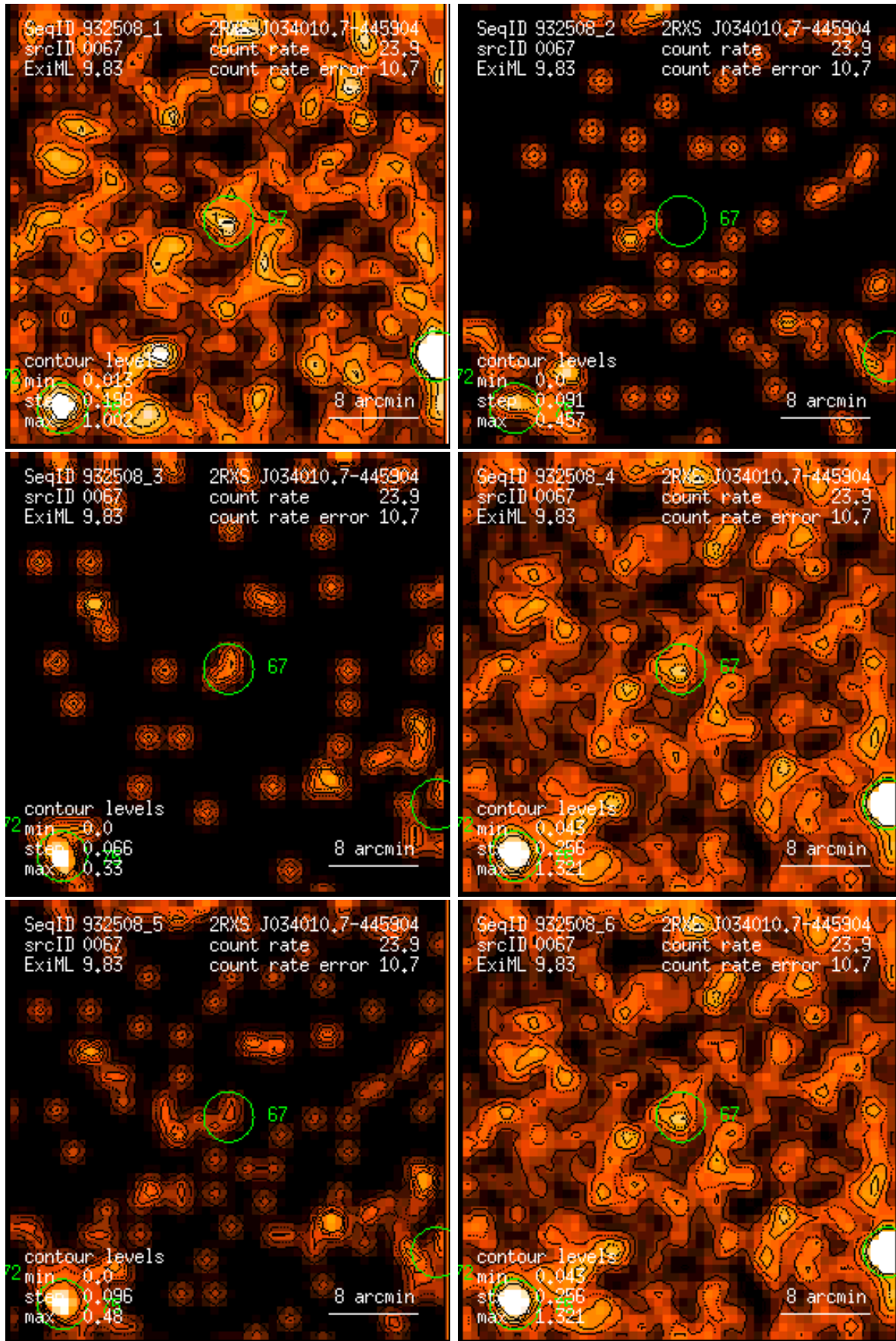
Figure 67: RASS 932508: detection 0067: band rate images, Gaussian filter: (1) PSPC channels 11 – 41, (2) 52 – 90, (3) 91 – 201, (4) 11 – 235, (5) 52 – 201, (6) 11 – 201. Broad band rates in counts/ks. Band rate contour levels in counts/ks/arcmin 2 .
