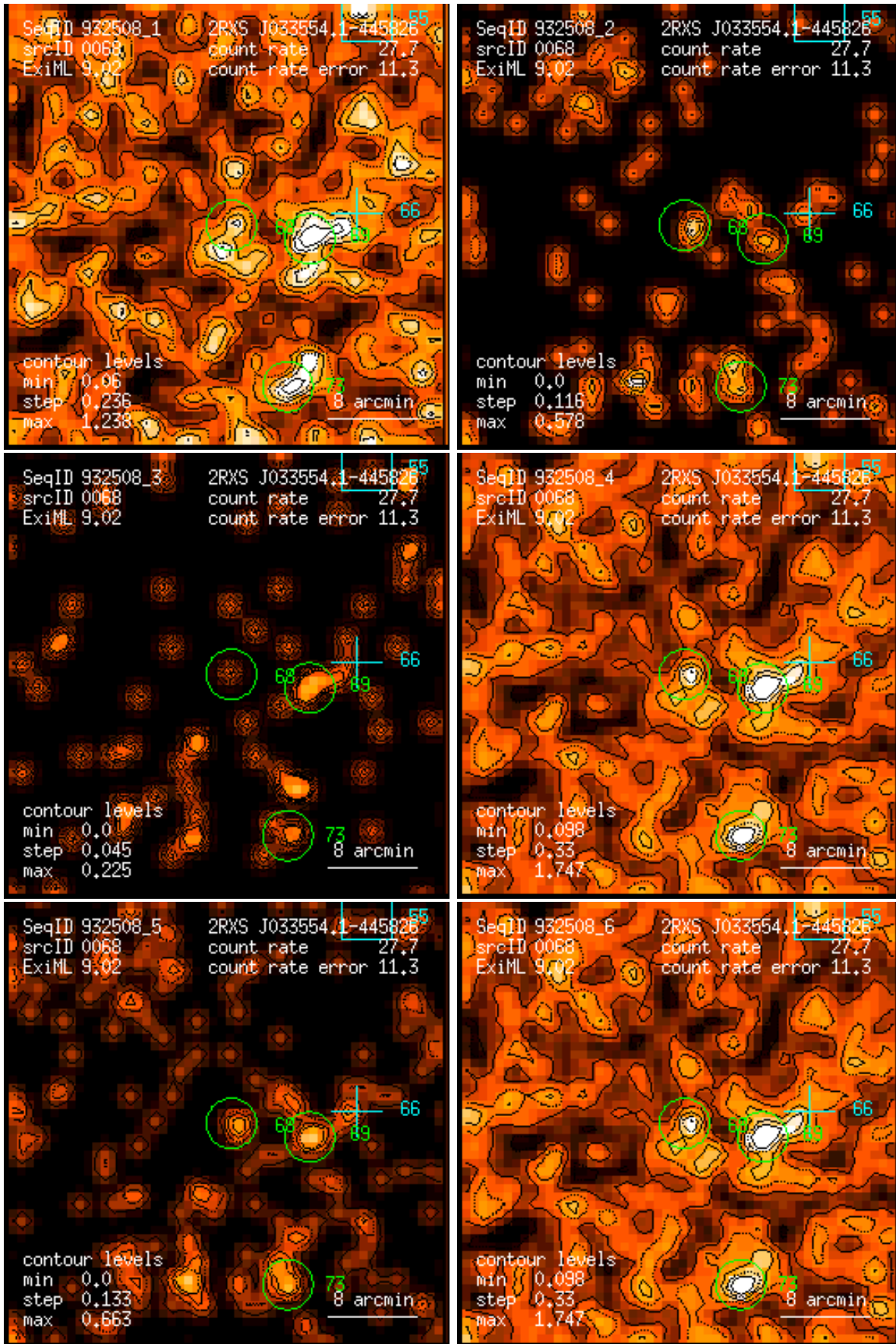
Figure 68: RASS 932508: detection 0068: band rate images, Gaussian filter: (1) PSPC channels 11 – 41, (2) 52 – 90, (3) 91 – 201, (4) 11 – 235, (5) 52 – 201, (6) 11 – 201. Broad band rates in counts/ks. Band rate contour levels in counts/ks/arcmin 2 .
