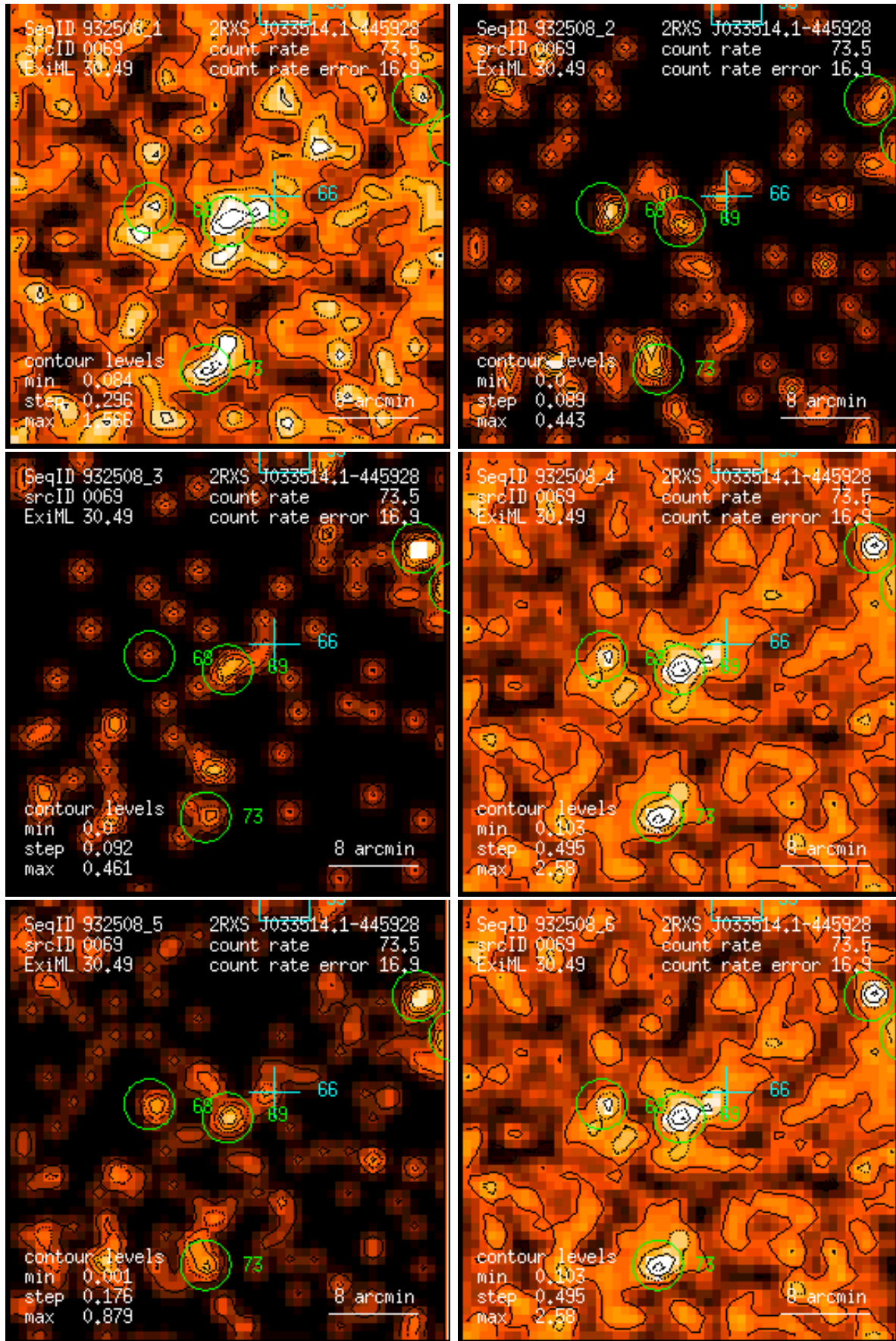
Figure 69: RASS 932508: detection 0069: band rate images, Gaussian filter: (1) PSPC channels 11 – 41, (2) 52 – 90, (3) 91 – 201, (4) 11 – 235, (5) 52 – 201, (6) 11 – 201. Broad band rates in counts/ks. Band rate contour levels in counts/ks/arcmin 2 .
