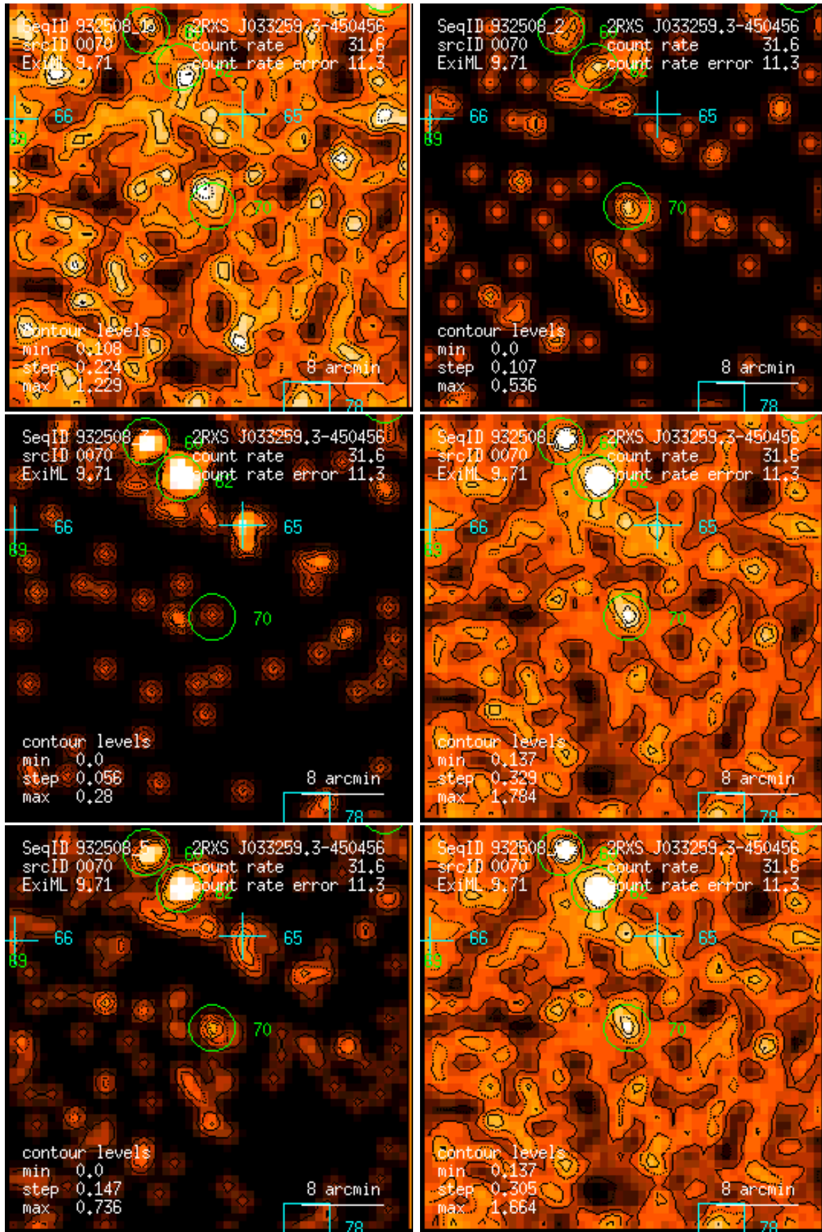
Figure 70: RASS 932508: detection 0070: band rate images, Gaussian filter: (1) PSPC channels 11 – 41, (2) 52 – 90, (3) 91 – 201, (4) 11 – 235, (5) 52 – 201, (6) 11 – 201. Broad band rates in counts/ks. Band rate contour levels in counts/ks/arcmin 2 .
