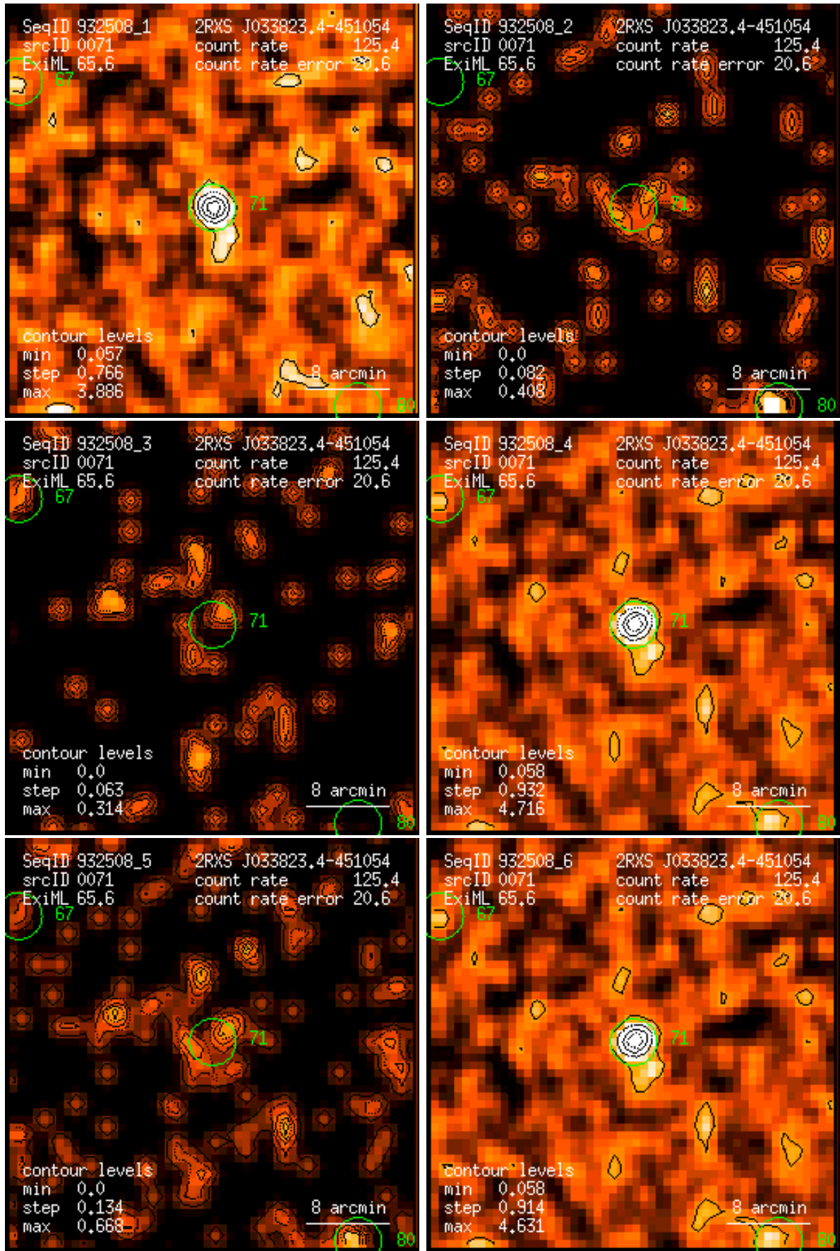
Figure 71: RASS 932508: detection 0071: band rate images, Gaussian filter: (1) PSPC channels 11 – 41, (2) 52 – 90, (3) 91 – 201, (4) 11 – 235, (5) 52 – 201, (6) 11 – 201. Broad band rates in counts/ks. Band rate contour levels in counts/ks/arcmin 2 .
