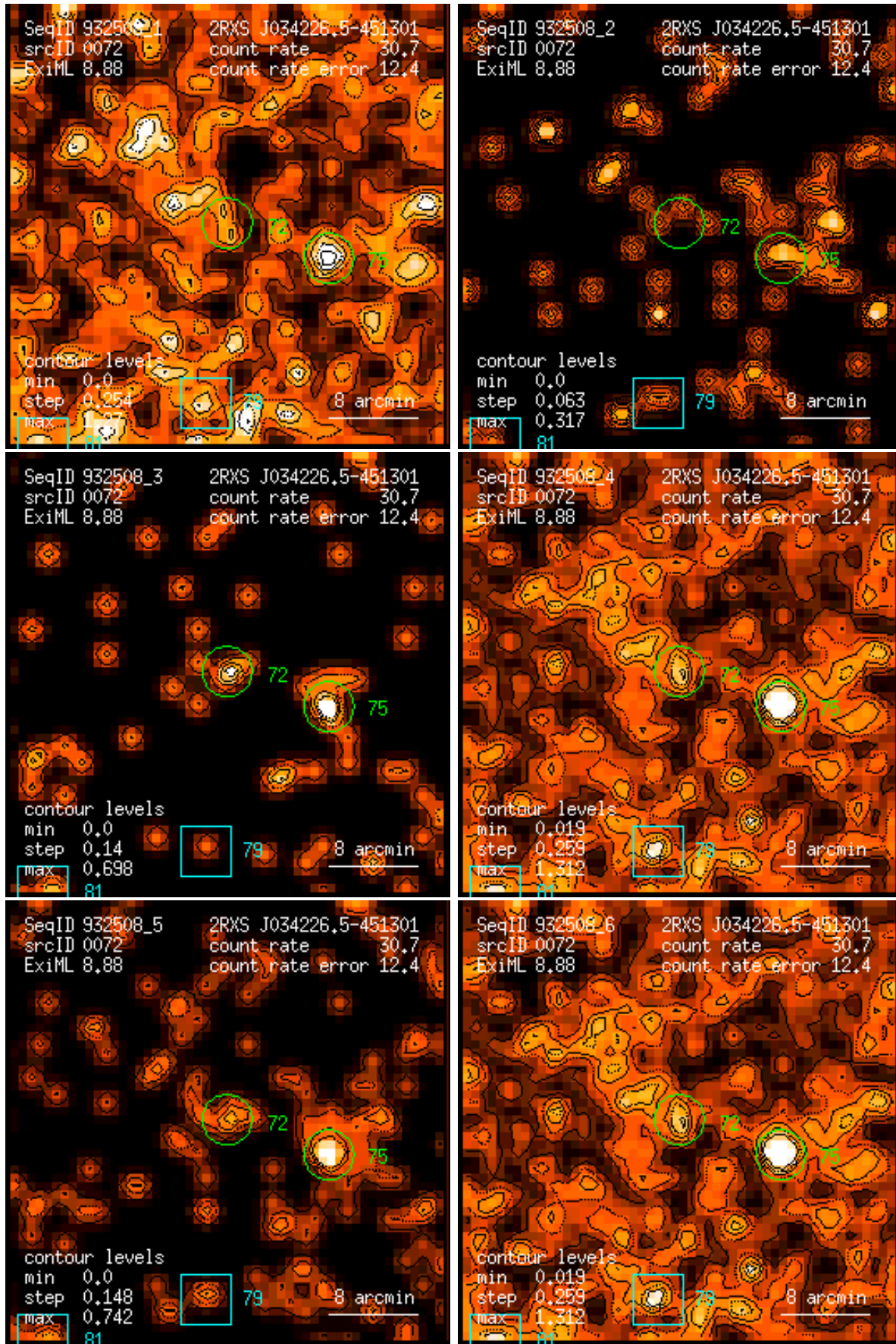
Figure 72: RASS 932508: detection 0072: band rate images, Gaussian filter: (1) PSPC channels 11 – 41, (2) 52 – 90, (3) 91 – 201, (4) 11 – 235, (5) 52 – 201, (6) 11 – 201. Broad band rates in counts/ks. Band rate contour levels in counts/ks/arcmin 2 .
