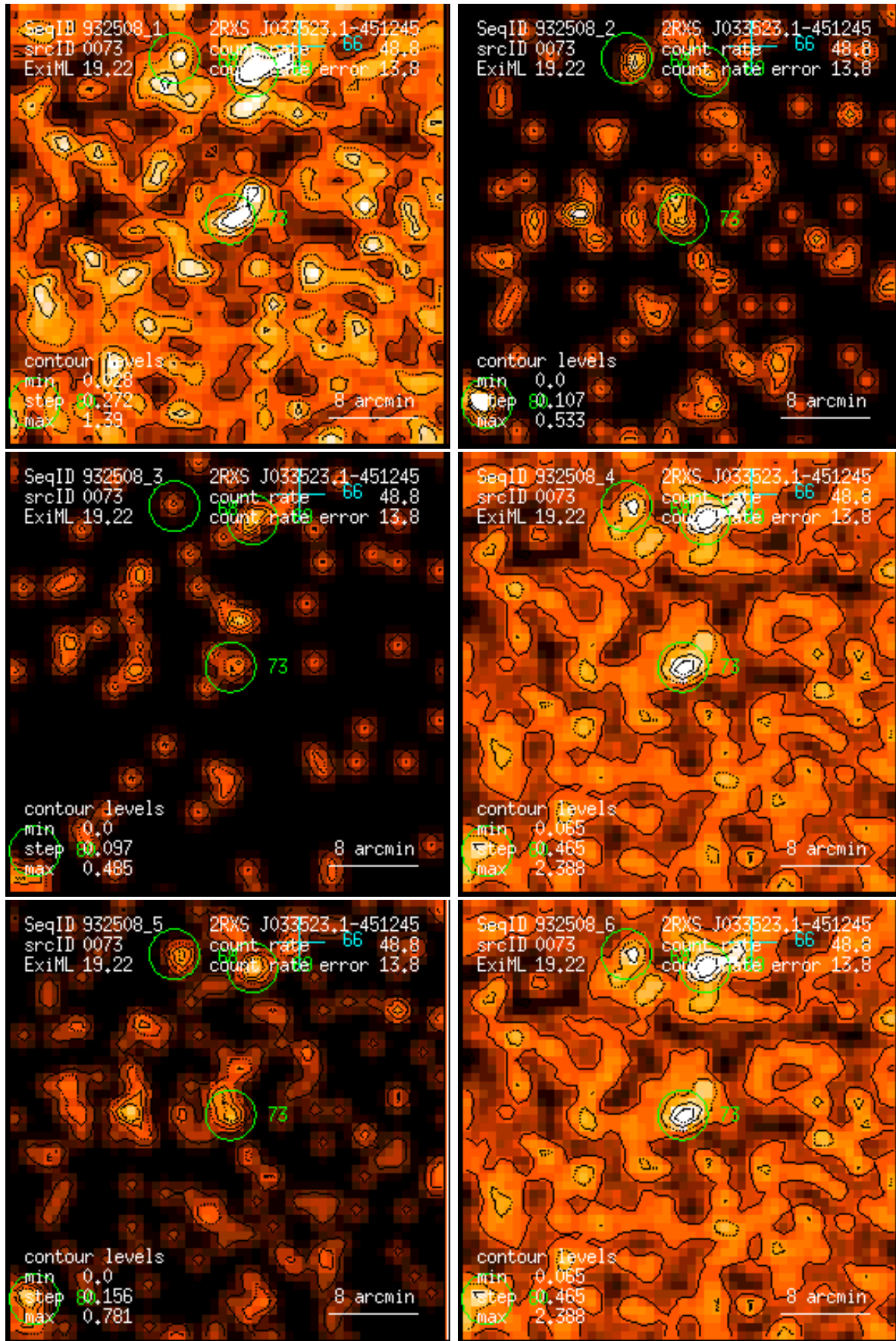
Figure 73: RASS 932508: detection 0073: band rate images, Gaussian filter: (1) PSPC channels 11 – 41, (2) 52 – 90, (3) 91 – 201, (4) 11 – 235, (5) 52 – 201, (6) 11 – 201. Broad band rates in counts/ks. Band rate contour levels in counts/ks/arcmin 2 .
