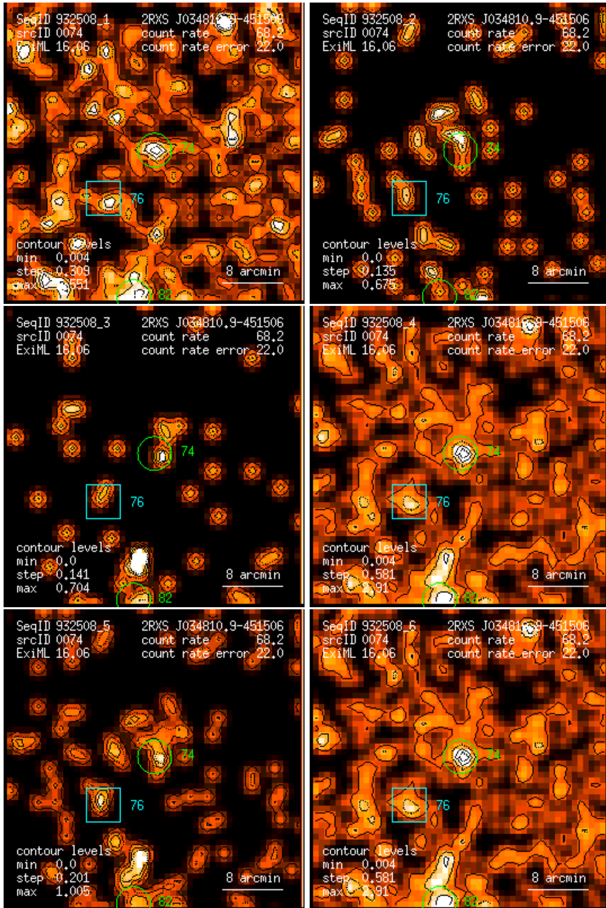
Figure 74: RASS 932508: detection 0074: band rate images, Gaussian filter: (1) PSPC channels 11 – 41, (2) 52 – 90, (3) 91 – 201, (4) 11 – 235, (5) 52 – 201, (6) 11 – 201. Broad band rates in counts/ks. Band rate contour levels in counts/ks/arcmin 2 .
